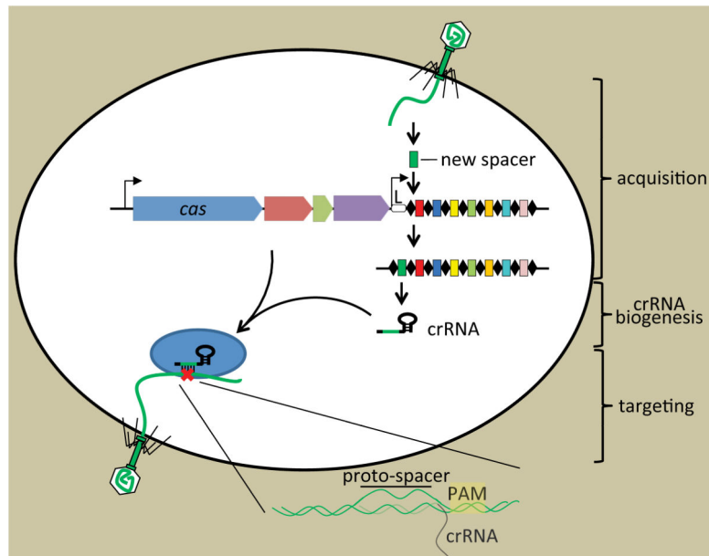
Figure 1. The three stages of CRISPR immunity
