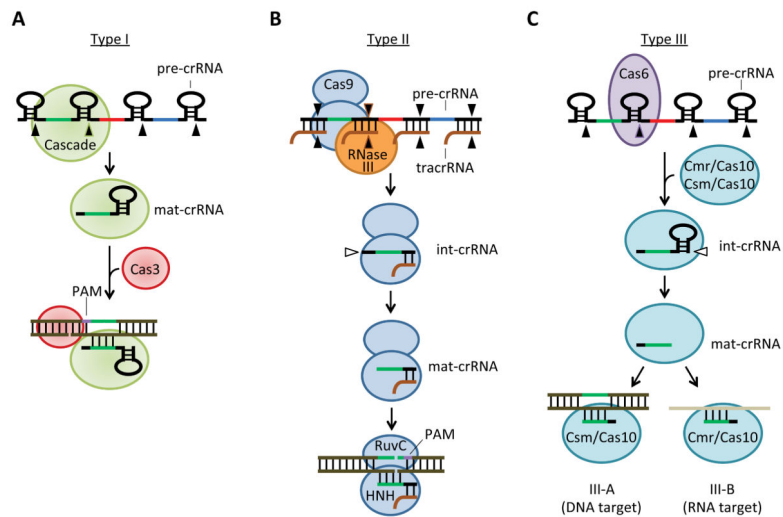
Figure 2. Mechanism of crRNA biogenesis and targeting in the three Types of CRISPR-Cas systems
