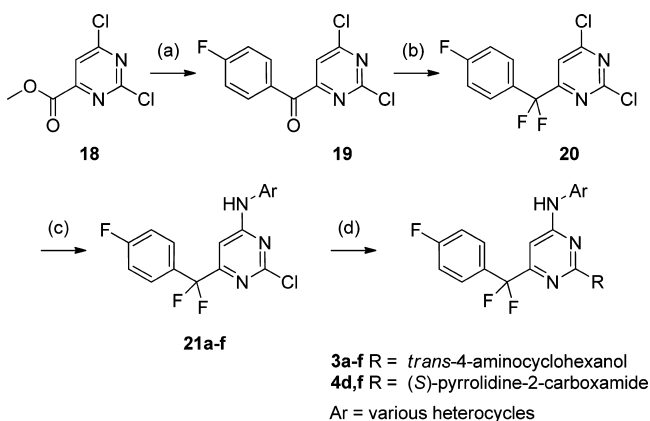
Scheme 1 a
