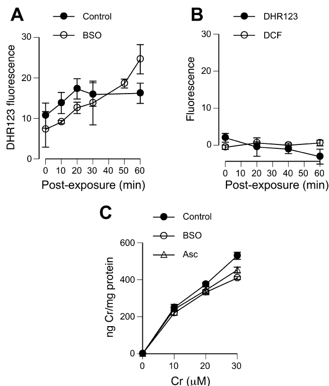
Figure 7. DHR123 and DCF fluorescence in Cr(VI)-treated H460 cells. Cells were preloaded with 10 \mu\text{M} dye for 30 min prior to a 1-h long treatment with 20 \mu\text{M} Cr(VI). Data are the means \pm SD ( n = 3 ). (A) Background-subtracted DHR123 fluorescence at different times after Cr removal. BSO cells were treated with 0.2 mM BSO for 24 h to deplete GSH. (B) Background-subtracted DCF and DHR123 fluorescence in Asc-restored cells treated with 30 \mu\text{M} Cr(VI). (C) Cr(VI) uptake by control and Asc-restored cells.
