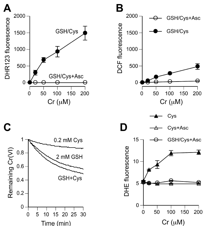
Figure 6. Responses of DHR123, DCF, and DHE in Cr(VI) reactions with Asc-thiol mixtures. Fluorescence was recorded after 30 min incubations and adjusted for the amount of Cr(VI) reduction. Shown are the means \pm SD, n = 3 . (A) DHR123 fluorescence and (B) DCF fluorescence in reactions containing 2 mM GSH and 0.2 mM Cys (GSH/Cys label) or both thiols plus 2 mM Asc (GSH/Cys + Asc label). (C) Kinetics of Cr(VI) reduction by 0.2 mM Cys, 2 mM GSH, and their mixture. (D) DHE fluorescence in Cr(VI) reactions with 2 mM Cys (Cys label), 2 mM Cys and 2 mM Asc (Cys + Asc label), or 2 mM GSH, Cys, and Asc (GSH/Cys + Asc label).
