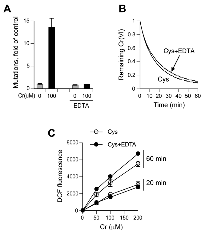
Figure 3. Cr(III) chelation by EDTA blocks the formation of mutagenic DNA damage by Cr(VI). (A) Mutagenic responses in pSP189 plasmids incubated in Cr(VI) reactions with 2 mM Cys in the absence or presence of 2 mM EDTA. Data are the means \pm SD from two experiments. (B) Kinetics of Cr(VI) reduction by 2 mM Cys with and without 2 mM EDTA. (C) DCF fluorescence in Cr(VI)-Cys reactions lacking or containing 2 mM EDTA. Measurements were taken after 20 and 60 min incubations. Data are the means \pm SD, n = 3 . Where not visible, error bars were smaller than symbols.
