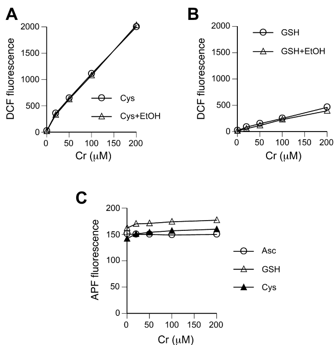
Figure 2. Testing for \text{OH}\cdot radicals in Cr(VI)-reducer reactions. Samples were incubated for 60 min with 2 mM Cys or GSH. Fluorescence was normalized for the amount of reduced Cr(VI). (A) No effect of ethanol on DCF fluorescence in Cr(VI)-Cys and (B) Cr(VI)-GSH reactions (EtOH, 1 mM ethanol). Data are the means for three measurements. Error bars are not shown for clarity. (C) Fluorescence of the highly reactive species indicator APF. Shown are the means for three determinations.
