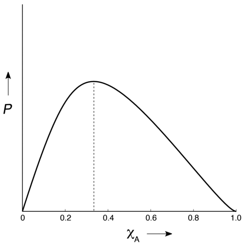
Figure 5. Job plot showing a 2:1 binding stoichiometry (eq 4) for an AB 2 complex.
