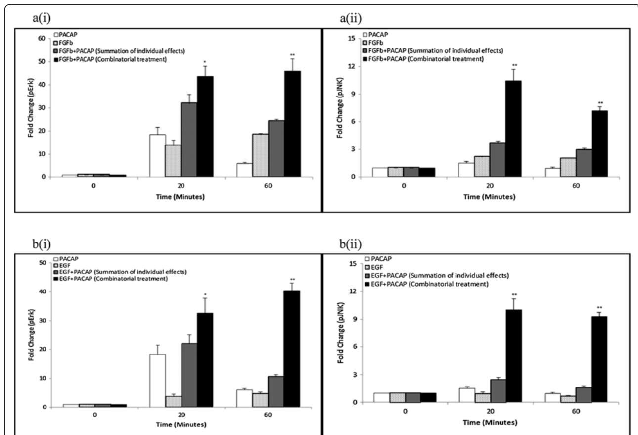
Figure 3 Synergistic and sustained phosphorylation of Erk and JNK upon FP and EP treatments. Time-course of quantified Erk and JNK phosphorylation at 20 and 60 minutes upon (a) FGFb (50 ng/ml)-PACAP (100 ng/ml) (FP) or (b) EGF (50 ng/ml)-PACAP (100 ng/ml) (EP) treatment. Fold-change in (i) pErk, and (ii) pJNK were quantified by densitometry and normalized to the levels of actin. Significant differences between combinatorial experimental treatment of growth factor-PACAP and the summation of their individual effects were calculated using the paired Student's t-test. A value of p < 0.05 was considered significant (** p < 0.01 ; * p < 0.05 ).
