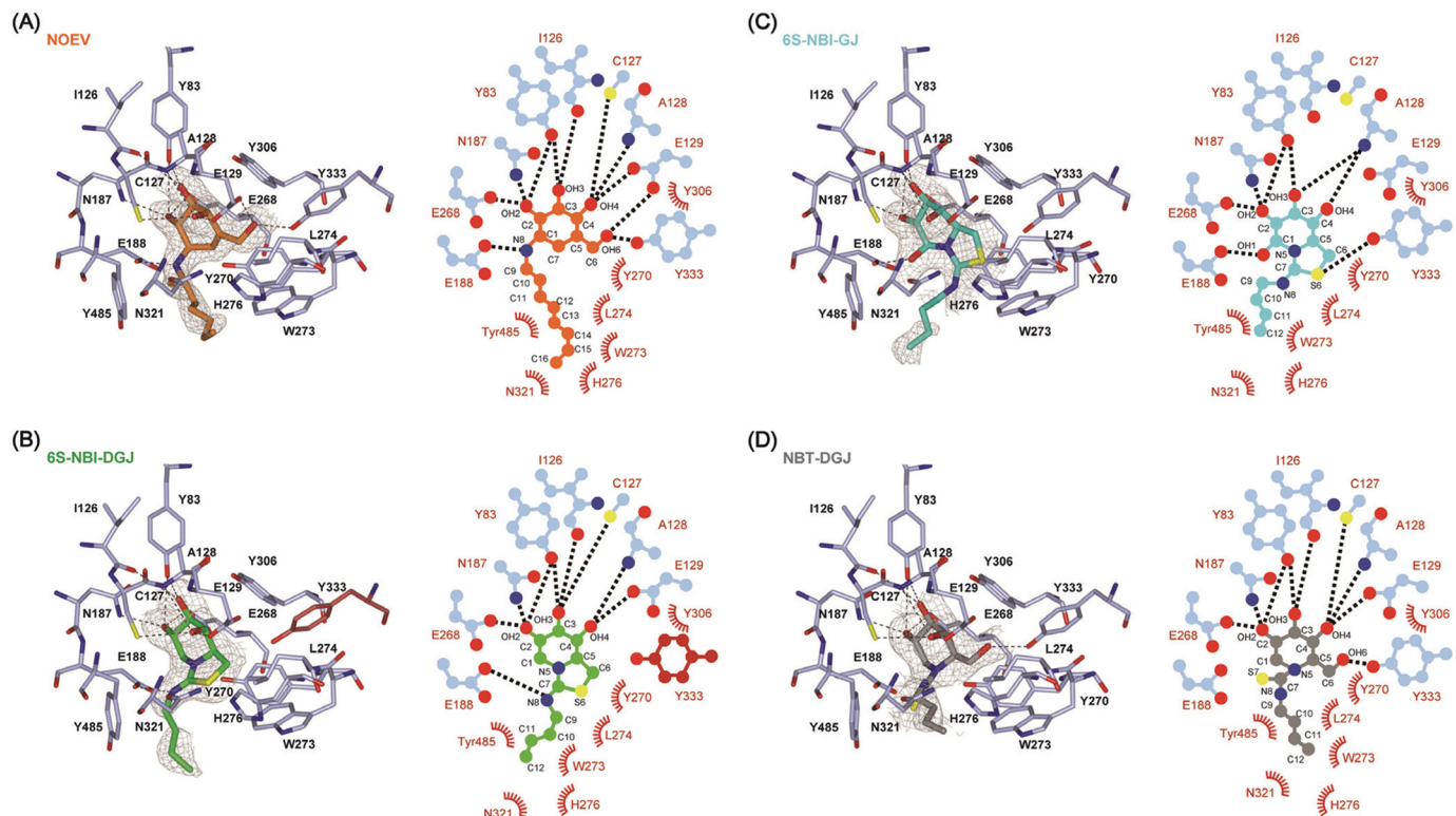
FIGURE 4. Binding of PC compounds to the active site of human \beta -Gal. A–D, left, PC compounds bound to \beta -Gal viewed from the entrance of active site pocket: A, NOEV; B, 6S-NBI-DGJ; C, 6S-NBI-GJ; D, NBT-DGJ. Hydrogen bonds defined by ccp4 mg (37) are shown by dashed lines. In B, a unique side chain arrangement of Tyr-333 in the 6S-NBI-DGJ complex is shown in crimson. The F_o - F_c electron density maps of PC compounds are shown in gray. A and B are contoured at 2.0 \sigma , C at 1.0 \sigma , and D at 1.5 \sigma . Right, schematic representation of the interaction between \beta -Gal and each PC compound: A, NOEV; B, 6S-NBI-DGJ; C, 6S-NBI-GJ; and D, NBT-DGJ. Hydrogen bonds are shown as dotted lines, and van der Waals interactions are shown by arcs.
