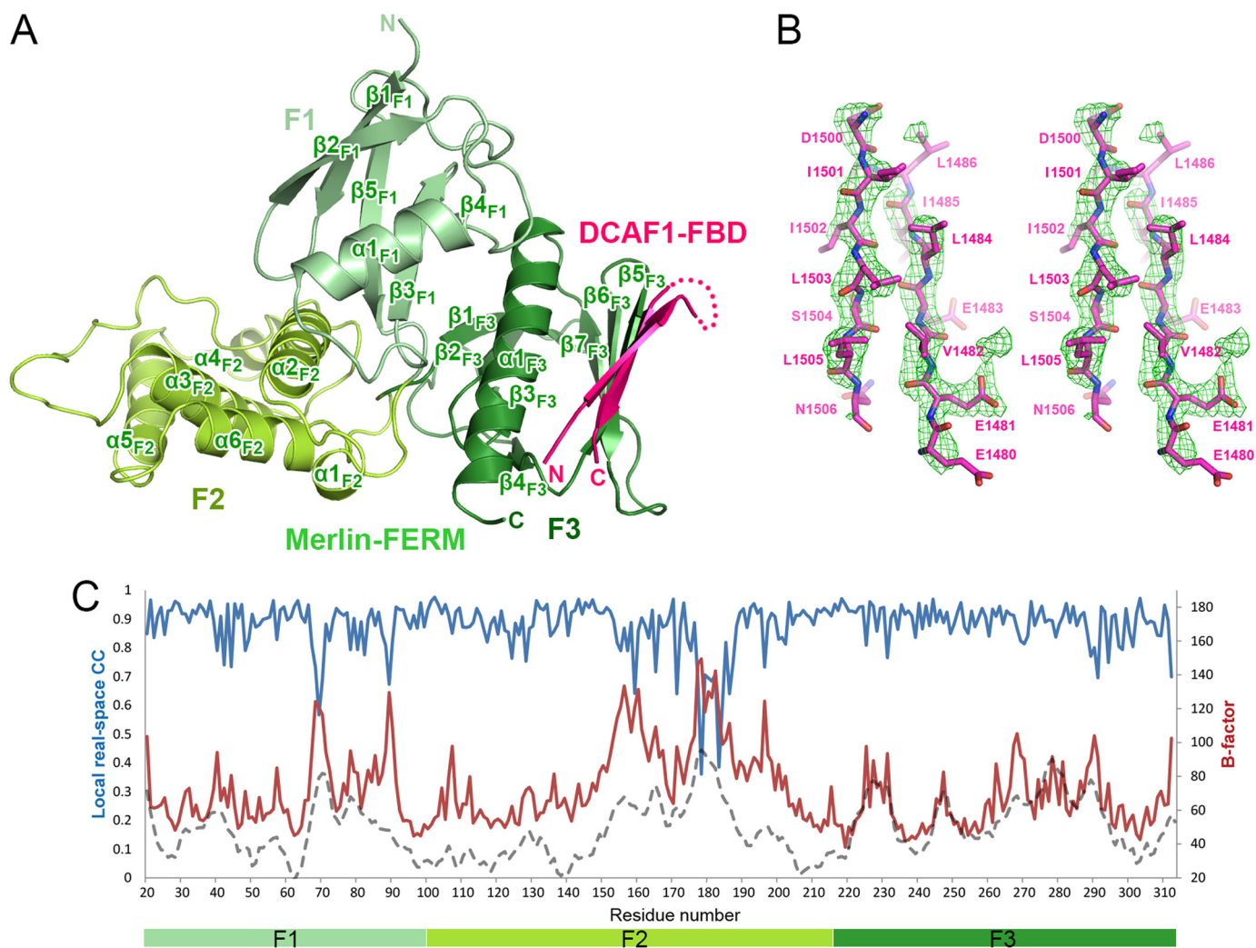
FIGURE 2. Overall structure of the Merlin-FERM-DCAF1-FBD complex. A , the crystal structure is presented as a ribbon diagram with the three lobes of Merlin-FERM, F1 (light green), F2 (green), F3 (dark green), and DCAF1-FBD (pink) drawn in their specific colors. The same color code is used throughout the rest of the figures except as otherwise indicated. The disordered loop connecting two \beta -strands is indicated by a dotted line. B , the simulated annealing omit map (green mesh) for the DCAF1-FBD hairpin structure. The map was contoured at 3\sigma with the structural model superimposed. C , the B-factor (red curve) and real-space (blue curve) correlation plot of Merlin-FERM in our crystal structure. The B-factor distribution (gray dashed curve) of the apo Merlin-FERM structure (Protein Data Bank code 11SN) was shown for comparison.
