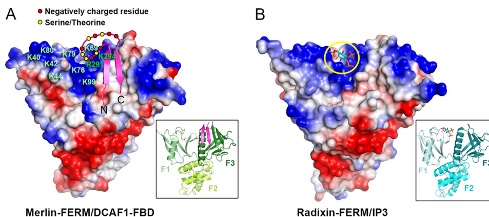
FIGURE 4. The negatively charged connecting loop of the DCAF1-FBD \beta -hairpin contributes to the binding to Merlin-FERM. A , the model of the connecting loop interacting with the highly positively charged F1/F3 cleft on Merlin-FERM. The figure was drawn using an electrostatic surface charge potential map with blue for the positive charge potential and red for the negative charge potential. The positively charged residues involved in forming the cleft are labeled. B , the structure of the FERM domain of Radixin in complex with the headgroup of phosphatidylinositol 4,5-bisphosphate (Protein Data Bank code 1GC6) was shown in the same presentation mode as A for comparison. The headgroup structure is highlighted by a yellow circle.
