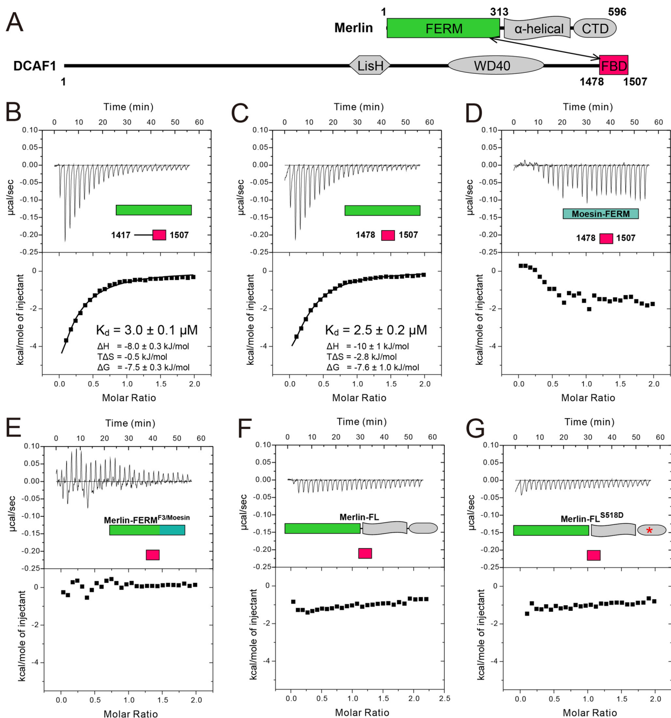
FIGURE 1. Characterization of the Merlin-FERM/DCAF1 interaction. A, domain organizations of Merlin and DCAF1 are shown as schemes. The Merlin-FERM/DCAF1-FBD interaction is indicated by a double-headed arrow . B–G, ITC-based measurements showing the binding affinities between DCAF1-CT and Merlin-FERM (B), and between DCAF1-FBD and Merlin-FERM (C), Moesin-FERM (D), Merlin-FERM F3/Moesin (E), Merlin-FL (F), and Merlin-FL S518D (G).
