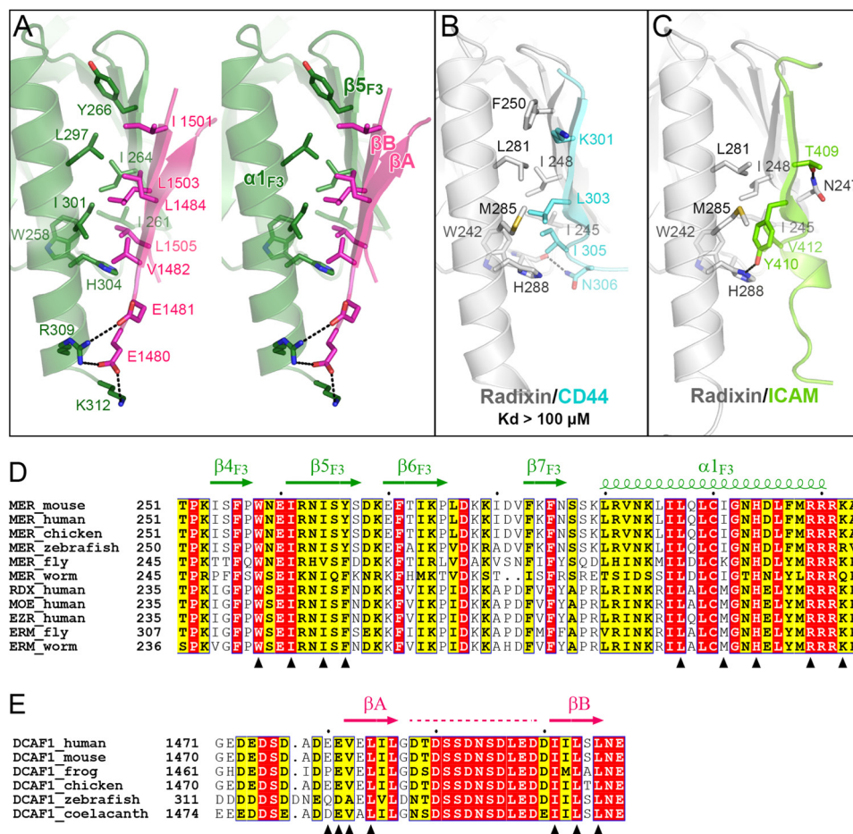
FIGURE 3. Structural and sequence analysis of the Merlin-FERM/DCAF1-FBD interaction. A , molecular details of the Merlin-FERM/DCAF1-FBD interaction. The residues involved in forming the FERM/FBD interface are shown as sticks. Hydrogen bonds and salt bridges are indicated by dashed lines . B and C , two examples showing that CD44 (Protein Data Bank code 2ZPY) and ICAM-2 (Protein Data Bank code 1J19) bind to the \alpha\beta -groove in the F3 lobe of Radixin (an ERM protein) as the single \beta -strand structures. We also measured the binding between the CD44 peptide and Moesin-FERM by ITC and found that their interaction is very weak ( K_d > 100 \mu\text{M} ). D , sequence alignment of the \alpha\beta -groove region in the FERM domains from Merlin and ERM family members. E , sequence alignment of the FBD regions from DCAF1 proteins across different species. In these two alignments, residues that are absolutely conserved and highly conserved are highlighted in red and yellow , respectively. The secondary structural elements are indicated above the alignments. The residues shown in Fig. 3 A are indicated by triangles in D and E , respectively. The disordered region in DCAF1-FBD is indicated by a dashed line in E .
