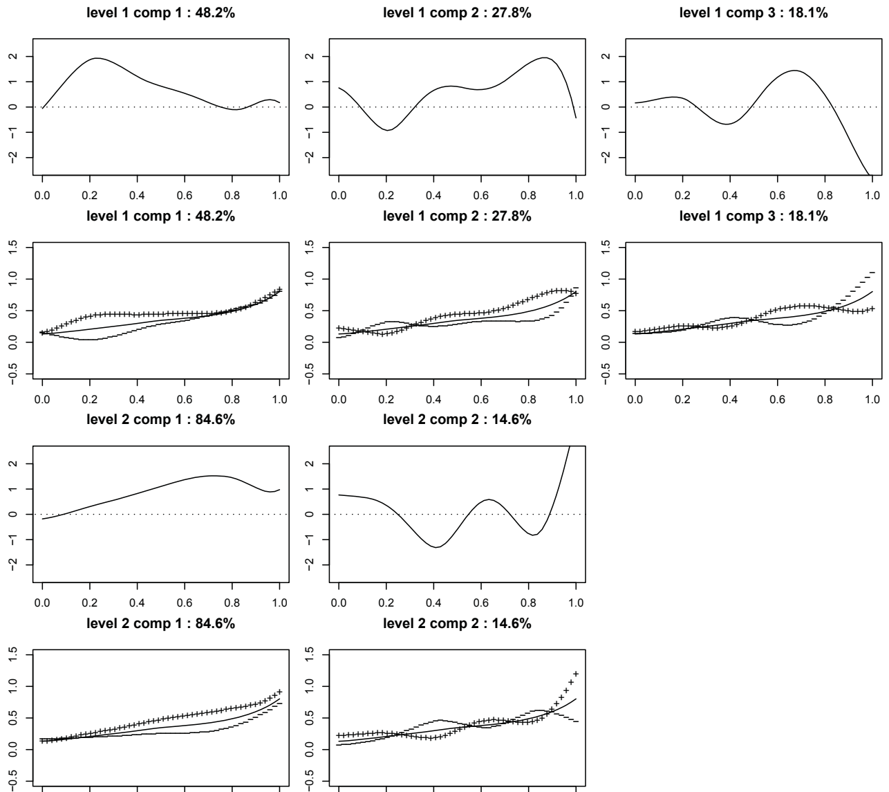
Figure 6. Estimated eigenfunctions at level 1 (Rows 1-2) and level 2 (Rows 3-4). In Row 1 and 3, the solid lines represent estimated eigenfunctions. In Row 2 and 4, solid lines represent the overall mean function \mu(t) , and the lines indicated by "+" and "-" are mean function plus or minus a multiple of \phi_1^{(1)}(t) , respectively. Namely, "+" represents \mu(t) + c\phi_1^{(1)}(t) , and "-" represents \mu(t) - c\phi_1^{(1)}(t) for some constant c .
