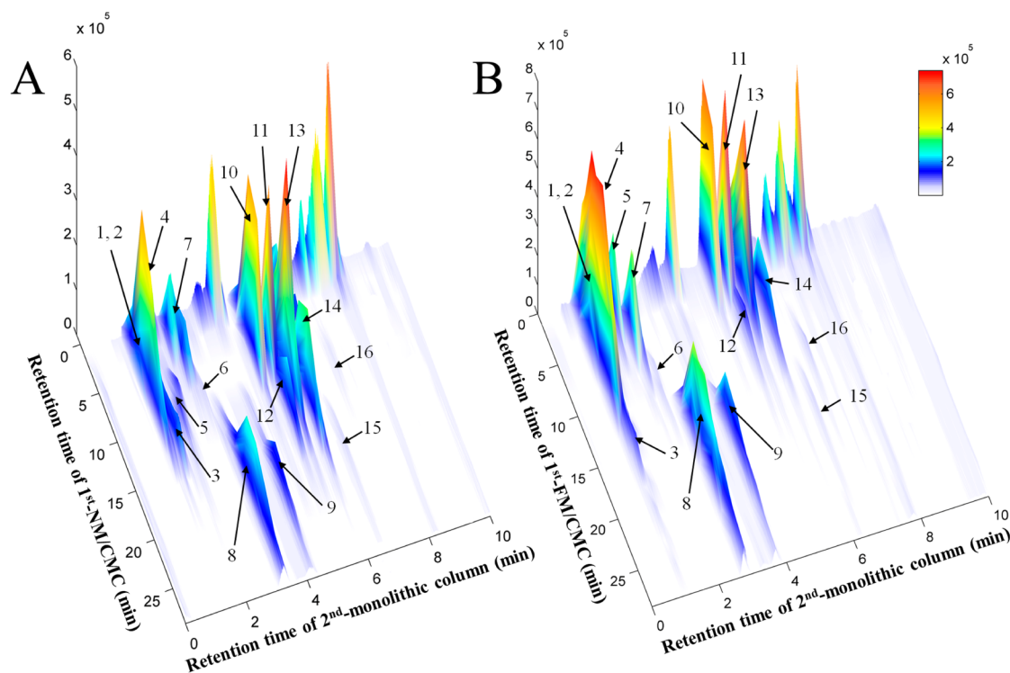
Figure 3. 3D plots of Fuzi extracts obtained by the comprehensive 2D (A) NM/CMC and (B) FM/CMC combined with monolithic column/TOFMS system. 1D: NM/CMC column (10 mm × 2 mm i.d.); Injection volume, 5 \mu L of Fuzi extract (0.3 g crude drug/mL); Flow rate, 0.2 mL/min; Mobile phase, 5 mM ammonia acetate; Temperature, 37 ^{\circ} C. 2D: monolithic column (100 mm × 4.6 mm i.d.); Mobile phase, 0.1% formic acid (v/v) and acetonitrile; Gradient elution: 0–5 min, from 5% ACN to 25% ACN; 5–9 min, from 25% ACN to 75% ACN; 9–4.5 min, from 75% ACN to 5% ACN; 9.5–10 min, 5% ACN; Flow rate, 3.5 mL/min; Temperature, 30 ^{\circ} C. For peak identification, see Table 1.
