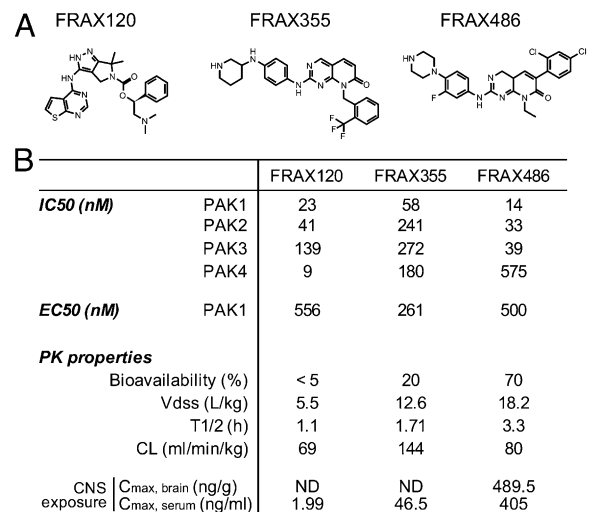
Fig. 2. Characteristics of PAK inhibitors. Chemical structure of three major compounds (A) and pharmacological properties (B).
