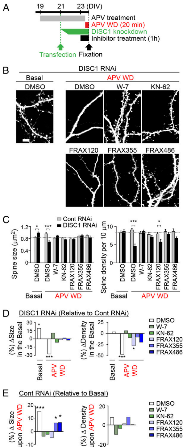
Fig. 3. Chemical inhibitors of PAK block DISC1 knockdown-elicited synaptic changes associated with NMDA-R activation. (A) Experimental design. Inhibitors with concentrations of 10 μM for W-7, 10 μM for KN-62, 250 nM for FRAX355, 500 nM for FRAX120, or 500 nM for FRAX486 were added 1 h before APV WD, followed by incubation of APV WD solution containing the inhibitor at same concentration for 20 min. (B–E) Morphometry spine analysis showing the effect of each compound on APV WD-induced spine structural change. The absolute values of spine size and density and the relative size and density after APV WD in the presence of each compound [ \Delta size (%) and \Delta density (%)] are shown. Beneficial effects of PAK inhibitors to the shrinkage of spine size were shown. In particular, FRAX355 and FRAX486 displayed beneficial influences on spine density without robustly affecting synaptic plasticity. **P < 0.01 . ***P < 0.001 . (Scale bar, 5 μm.)
