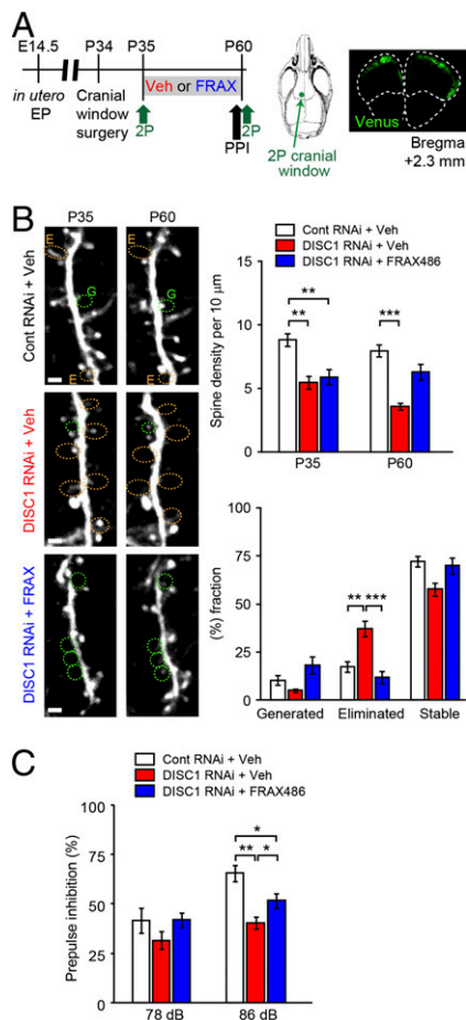
Fig. 6. The PAK inhibitor (FRAX486) ameliorates adolescent synapse loss in the prefrontal cortex and adult behavior change in a DISC1 knockdown mouse model. (A) Experimental design. DISC1 or control shRNA was transferred at embryonic day 14.5 (E14.5). Mice with shRNA were subjected to cranial window surgery at postnatal day 34 (P34). Two-photon imaging (2P) was performed both at P35 and P60. Location of cranial window and shRNA distribution (in green) at P60 were shown. Prepulse inhibition (PPI) was tested just before the two-photon imaging at P60. (B) Spine analyses. DISC1 shRNA led to a marked reduction in the spine density at both postnatal days 35 and 60 (P35 and P60), which was further augmented at P60 (** P < 0.01 ; *** P < 0.001 ). Daily administration of FRAX486, but not that of vehicle, between P35 and P60 blocked the exacerbated spine loss during adolescence. The effects of FRAX486 were significant in blocking spine elimination (** P < 0.001 ). In addition, a trend of enhanced spine generation ( P = 0.07 ) was observed by treatment with FRAX486. Spines surrounded by yellow and green dots indicate eliminated (indicated as E) and generated (indicated as G) spines between P35 and P60, respectively. (Scale bar, 2 μm.) (C) Performance in PPI at P60. Deficit in PPI in DISC1-knockdown mice was significantly, although partially, ameliorated by FRAX486 ( n = 12 per each group). * P < 0.05 , ** P < 0.01 .
