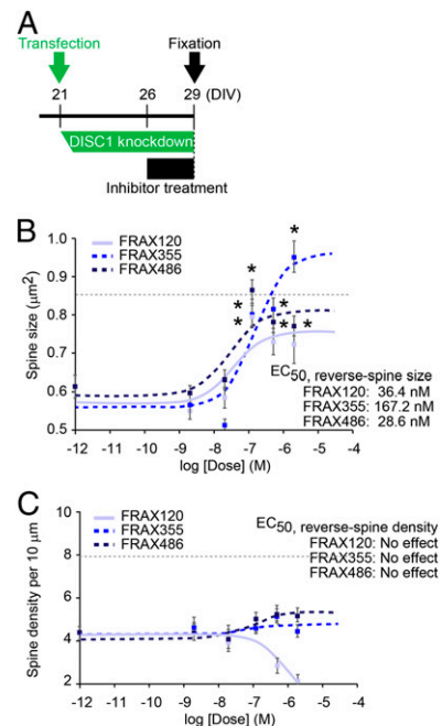
Fig. 5. Chemical inhibitors of PAK reverse already existing spine deterioration triggered by DISC1 RNAi (treatment effect). (A) Experimental design. PAK inhibitors were added 5 d after the transfection of either control or DISC1 RNAi, followed by 3 d incubation before fixation. (B and C) Dose–response curves of FRAX120, FRAX355, and FRAX486 for reversal effect on spine size (B) and spine density (C) in the neuron with DISC1 shRNA are shown. Asterisks indicate the significant differences between the spines with vehicle control and those with PAK inhibitor *P < 0.05 . The dotted lines indicate the average of the spine size (B) and the spine density (C) in cells with control shRNA (baselines). “Veh” indicates “Vehicle only” in dose–response curve. EC_{50} , half-maximum effective concentration in this treatment paradigm, is calculated.
