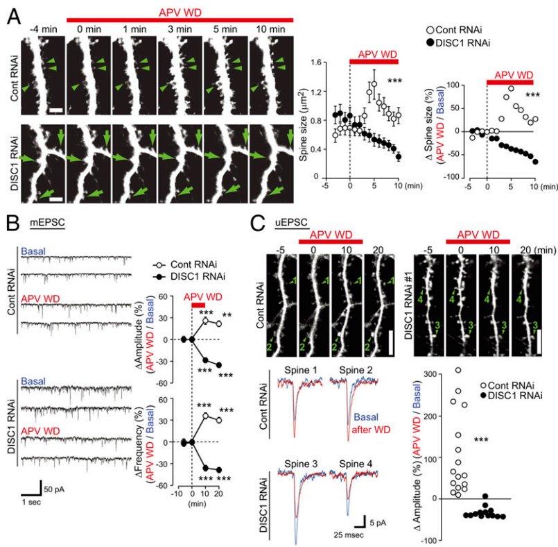
Fig. 1. DISC1 knockdown affects NMDA receptor (NMDA-R)-dependent synaptic plasticity. (A) Time lapse imaging showing structural plasticity of spine upon APV withdrawal (APV WD). Whereas spines on neurons with control shRNA (control RNAi, arrowheads) underwent spine enlargement, spines with DISC1 shRNA (DISC1 RNAi, arrows) were reduced in size upon NMDA-R activation. The absolute values of spine size and relative size upon APV WD are shown, which suggests that synaptic response between control and DISC1 RNAi-treated neuron are significantly different. (B) Changes of mEPSC upon APV WD in neurons with or without DISC1 RNAi. ^{**}P < 0.01 , ^{***}P < 0.001 compared with t = 0 min. (C) Changes of uEPSC showing functional plasticity upon APV WD in neurons with or without DISC1 RNAi. APV withdrawal induced spine enlargement and enhancement in synaptic transmission in control neuron (spines 1 and 2), whereas in contrast, there were spine shrinkage and reduction in synaptic transmission in DISC1 RNAi-treated neuron (spines 3 and 4). Changes in uEPSC amplitude ( \Delta amplitude) in each individual spine are shown (control RNAi, n = 16 ; DISC1 RNAi, n = 16 ). ^{***}P < 0.001 .
