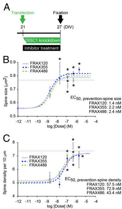
Fig. 4. PAK inhibitors prevent DISC1 RNAi-induced spine deterioration (prophylactic effect). (A) Experimental design. PAK inhibitors were added at the time of transfection for DISC1 RNAi and incubated for 6 d before fixation. (B and C) Dose–response curves of FRAX120, FRAX355, and FRAX486 for protective effects on the spine size (B) and spine density (C) in the neurons with DISC1 shRNA (DISC1 RNAi) are shown. Asterisks indicate significant differences between the spines with vehicle control and those with PAK inhibitor, which imply therapeutic effective dose of each compound *P < 0.05 . The dotted lines indicate the average of the spine size (B) and the spine density (C) in cells with control shRNA (baselines). “Veh” indicates “Vehicle only” in dose–response curve. EC_{50} , half-maximum effective concentration in this prophylactic paradigm, is calculated.
