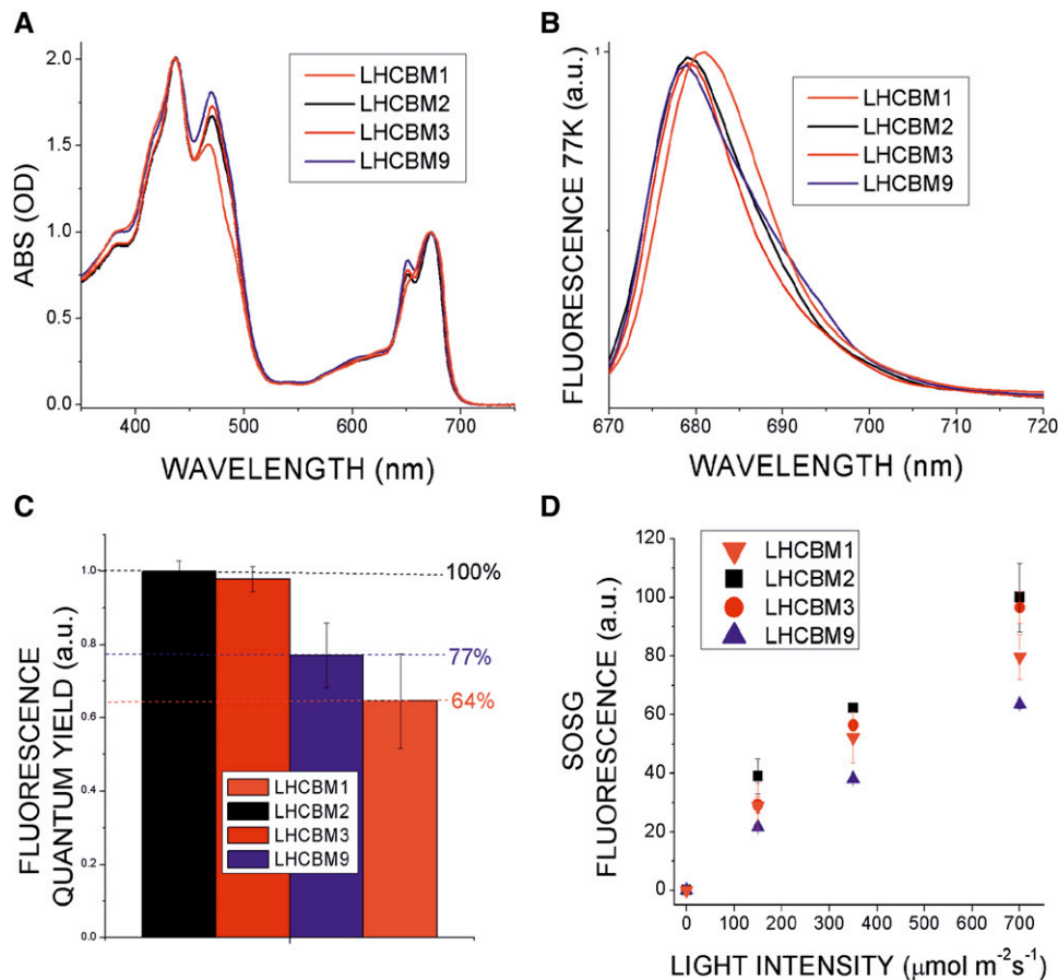
Figure 5. Spectroscopic Properties of LHCBM9 Compared with LHCBM1, 2, and 3.
