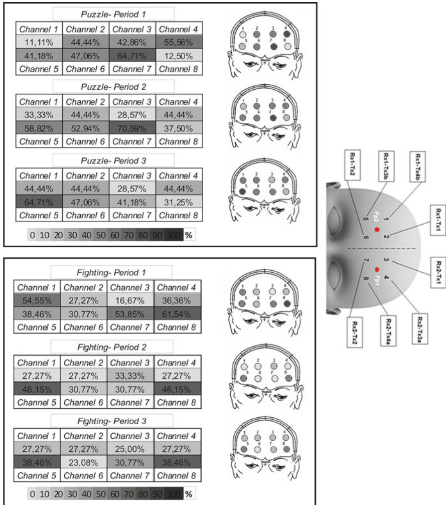
Fig. 13.1 Group analysis shows the percentage of subjects that demonstrated activation in specific channels and epochs
