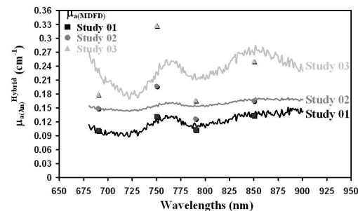
Fig. 3 Absolute broadband absorption from in-vivo muscle measurements in three volunteers during rest.
