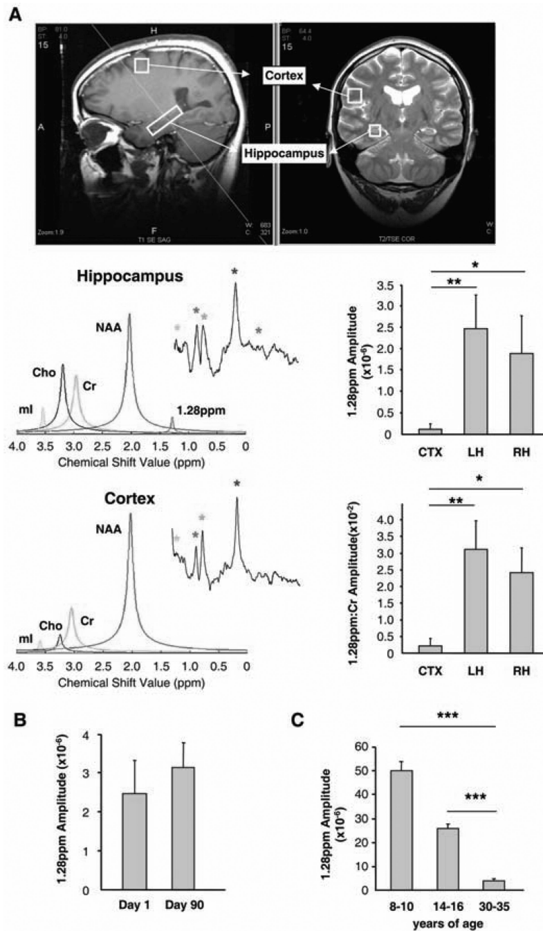
Fig. 4. Identification of NPCs in the human hippocampus in vivo, using ^1\text{H} -MRS. (A) Voxels are placed along the hippocampus and in the cortex. In the hippocampus, the 1.28-ppm biomarker (red) is evident when SVD-based signal processing is performed but not when Fourier transform is done. In the cortex, the 1.28-ppm biomarker is not detected by either data analysis. Colored asterisks and colored peaks correlate. Bar graphs show absolute (top) and relative (bottom) quantification of the 1.28-ppm biomarker (CTX, cortex; LH, left hippocampus; RH, right hippocampus; n = 5 people; P < 0.01 and P < 0.05 , respectively).
