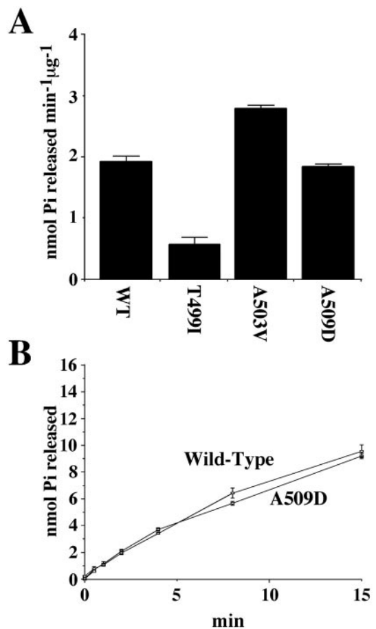
Figure 5. ATPase activities of proteins carrying single substitutions. Wild-type Hsp104p, Hsp104p T499I , Hsp104p A503V , and Hsp104p A509D proteins were purified from E. coli . (A) Basal ATP hydrolysis rates of each protein were assayed in a physiological salt buffer by release of Pi from ATP. (B) To establish that the similarity in ATP hydrolysis rates between Hsp104p A509D and wild-type Hsp104p is not restricted to early time points, they were compared over a range of time.
