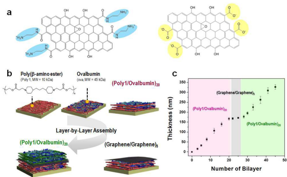
Figure 2. (a) Schematic representation of chemically modified graphene oxide GO-COO - and GO-NH 3 + . (b) Schematic illustrations of (\text{Poly1/ova})_{20}(\text{GO/GO})_5(\text{Poly1/ova})_{20} multilayer films. (c) Growth curve of electrostatically assembled (\text{Poly1/ova})_{20}(\text{GO/GO})_5(\text{Poly1/ova})_{20} multilayer films as a function of bilayer number.
