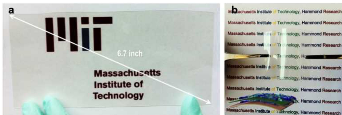
Figure 5. Photo images of thin film of substrate/(Poly1/ova-TR) 20 (GO/GO) 20 (Poly1/ova-FL) 20 multilayer film: (a) A large-area film transferred on a 6.7-inch PET sheet, (b) An assembled multilayer film showing outstanding flexibility.
