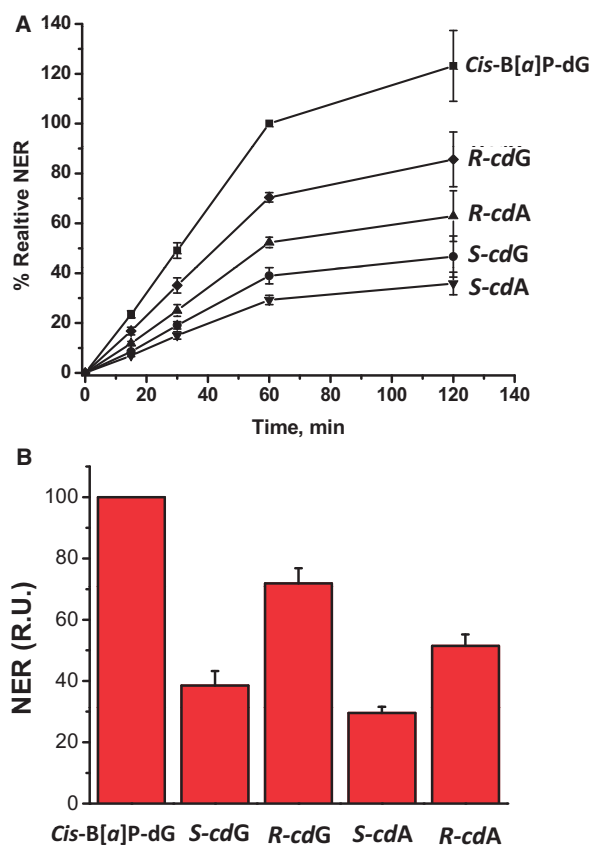
Figure 3. (A) Time course of NER dual incision product formation of 24–32 oligonucleotide fragments bearing either the cis-B[α]P-dG , 5′ R -cdG, 5′ R -cdA, 5′ S -cdG or 5′ S -cdA lesions. The experimental data points are averages of five independent experiments in different cell extracts, and the error bars represent the standard deviations. The incision efficiencies of the cdG- and cdA-containing sequences were normalized in each of the five independent experiments to the value obtained with cis-B[α]P-dG (relative value of 100 at the 60-min time point, also determined in each experiment). The results are thus provided in relative units (RU). The reaction kinetics are linear up to at least 60 min incubation times, and rates of reaction level off within the 60–120-min time interval. (B) Relative initial rates of dual incision kinetics determined by averaging the slopes of the straight line portions of the data obtained with the ODN(1) duplex (panel A), and the analogous plot obtained with the ODN(2) duplex (Supplementary Figure S3). The results obtained with the ODN(1) and ODN(2) duplexes were the same within experimental error (Supplementary Figure S3), and the 17-mer sequence contexts in which the cyclopurine lesions are embedded, are identical in ODN(1) and ODN(2).
