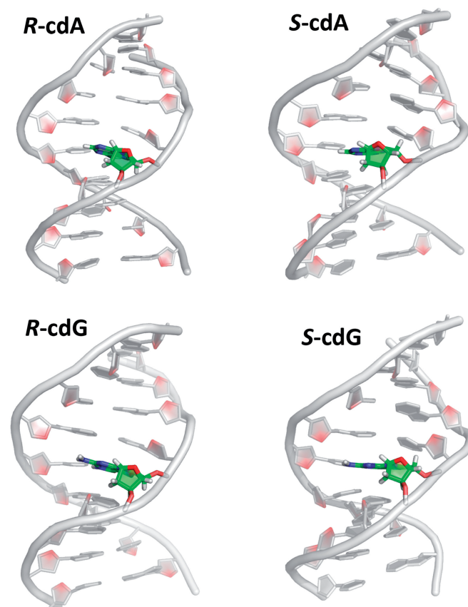
Figure 4. Central 9-mers of the best representative structures from the MD simulations of the 5′ R and 5′ S -cdA and cdG-containing 11-mer duplexes. Supplementary Figure S14 shows the corresponding unmodified controls.
