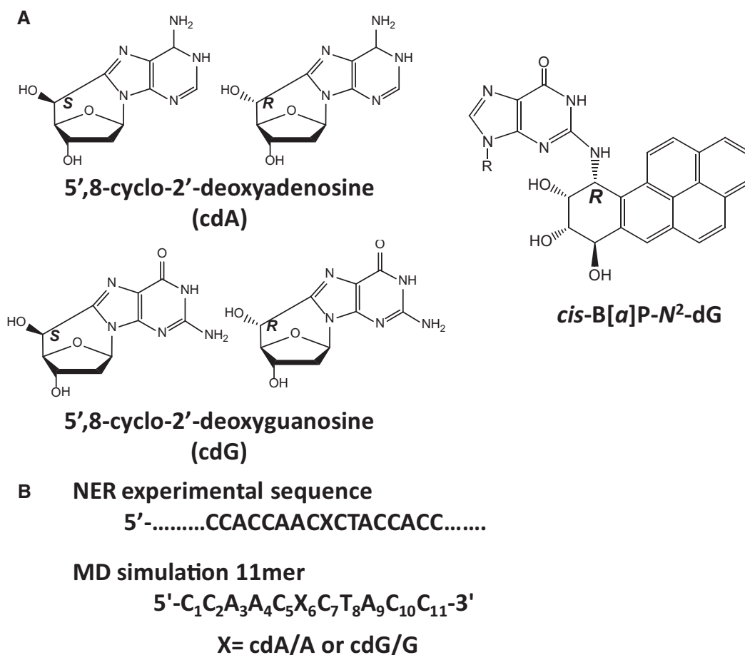
Figure 1. (A) Chemical structures of the cdA and cdG stereoisomeric lesions, together with the structure of the 10 R (+)- cis -B[a]P-N 2 -dG NER activity standard used to compare activities for cell extracts prepared at different times. (B) Sequences of the B-DNA duplexes used in the experimental and MD simulation studies. X denotes the modified site. For control simulations with unmodified duplexes, X = A or G. The complementary partner strands contain T opposite cdA/A and C opposite cdG/G.
