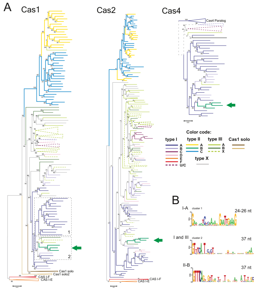
Figure 3. Origin of type II-B CRISPR-Cas system. (A) The PSI-BLAST program was used to retrieve Cas1 protein sequences from 2262 complete genomes in the Refseq database. The BLASTCLUST program (length coverage cutoff 0.8; score density threshold 1.0) was used to select 205 representative sequences. The multiple alignment was built using the MUSCLE program (see Supplementary Materials and Methods for details). The FastTree program ([Jones-Taylor-Thornton (JTT) evolutionary model, discrete gamma model for site rates with 20 rate categories; see Supplementary Materials and Methods for details]) was used for the tree reconstruction. The Cas2 and Cas4 phylogenetic trees were reconstructed using the FastTree program as indicated for the Cas1 tree above. The sequences of these families were chosen from the same genomic neighborhoods as the selected Cas1 representatives (a few incomplete sequences from both protein families were either omitted or replaced by closely related sequences from other species). Type II-B branches are indicated by the green arrow. The branches are colored according to the assignment of cas1 genes to CRISPR-Cas subtypes based on the analysis of 10 upstream and 10 downstream genes. X denotes systems of unknown type or those that are predicted to be derivatives of the respective system (when colored). The trees are shown only schematically, the complete trees are available in Supplementary Figure S2. (B) Logoplots of CRISPR repeats for the genomes that belong to several branches that are neighbors of the type II-B branch on the Cas1 phylogenetic tree. Clusters 1 and 2 are indicated by dashed lines. The type II-B (cluster 2) logoplot is shown separately. See details in Supplementary Figure S3.
