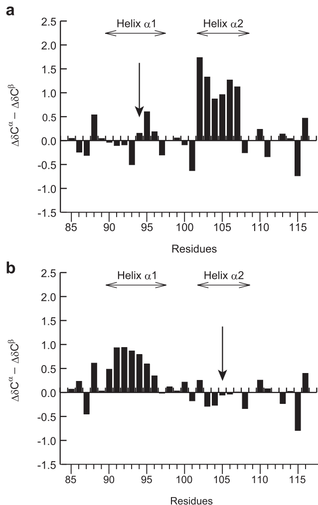
Figure 5 | \Delta\delta C^\alpha - \Delta\delta C^\beta secondary chemical shifts of the (a) L94P and (b) L105P mutant of RPEL1. The positions of helices \alpha 1 and \alpha 2 are indicated in each panel. The positions of the mutations are indicated by arrows.
