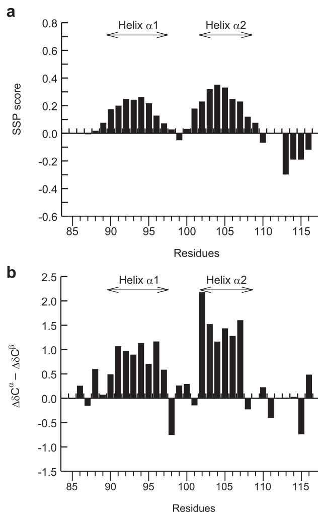
Figure 4 | (a) SSP scores of RPEL1. (b) \Delta\delta\text{C}^\alpha - \Delta\delta\text{C}^\beta secondary chemical shifts of RPEL1. The positions of helices \alpha 1 and \alpha 2 are indicated in each panel.
