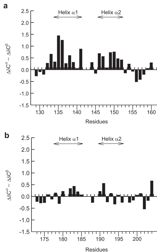
Figure 6 | \Delta\delta C^\alpha - \Delta\delta C^\beta secondary chemical shifts of (a) RPEL2 and (b) RPEL3. The positions of helices \alpha 1 and \alpha 2 are indicated in each panel.
