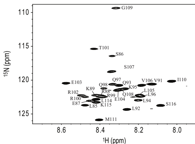
Figure 3 | The ^1\text{H} - ^{15}\text{N} HSQC spectrum of RPEL1 at pH 7.0 and 15^\circ\text{C} . The backbone resonance assignments are indicated. Numbering is based on GenBank accession number BAN82605.1.
