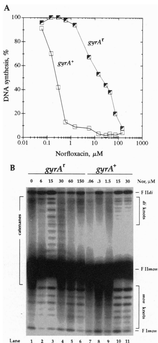
FIG. 1. (A) Norfloxacin inhibition of [ 3 H]thymidine incorporation into DNA in gyrA r (■) and gyrA + (□) strains. Cells were treated with drug for 15 min prior to the 1-min pulse with [ 3 H]thymidine. (B) Effect of norfloxacin on catenane accumulation. gyrA r (lanes 1–6) or gyrA + (lanes 7–11) strains were incubated with norfloxacin for 15 min at 37°C. Plasmid DNA was isolated and analyzed by agarose gel electrophoresis. Positions of supercoiled (F I), nicked (F II) monomer ( mon ) or dimer ( di ) rings, knots, and catenanes are shown.
