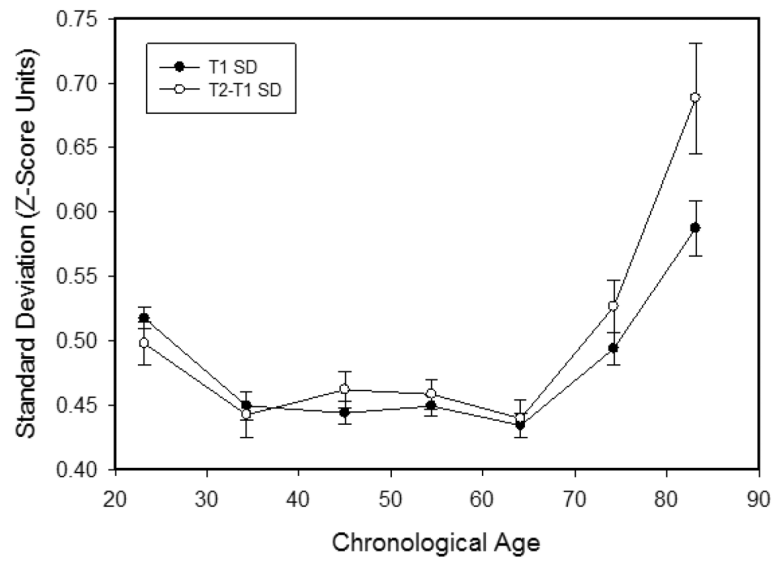
Figure 4. Means (and standard errors) of within-person standard deviations for vocabulary test scores at T1, and for the T2-T1 differences in vocabulary test scores by age decade.
