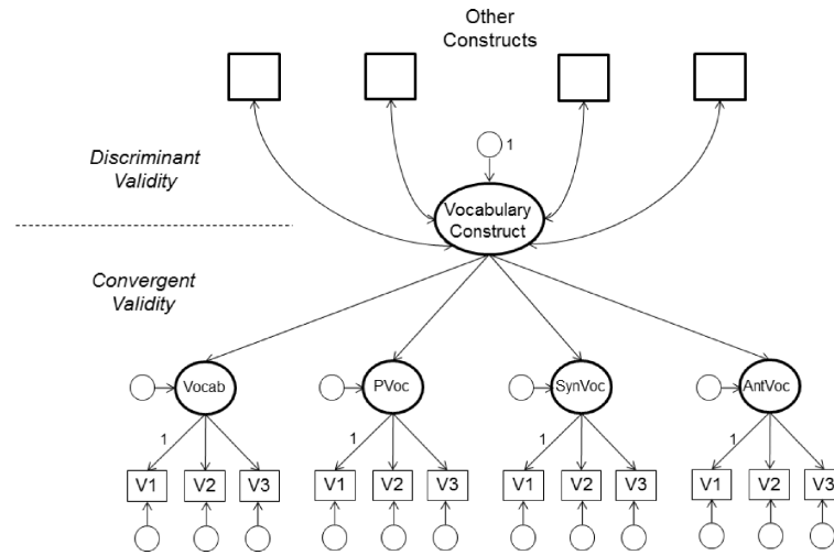
Figure 1. Schematic representation of a vocabulary construct defined by three versions in each of four tests. Vocab refers to WAIS Vocabulary, PVoc to Picture Vocabulary, Synvoc to synonym vocabulary, and Antvoc to antonym vocabulary. V1, V2, and V3 refer to different versions of tests with the same format but involving different items. Relations with ability constructs in the top panel are relevant to discriminant validity and relations of the vocabulary construct to the vocabulary test constructs, and of the test constructs to the test versions in the bottom panel are relevant to convergent validity.
