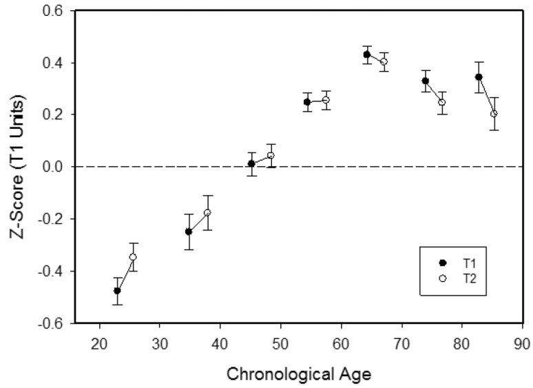
Figure 3. Means (and standard errors) of composite vocabulary scores for participants with data on the first session at both T1 and T2 by age decade. The T2-T1 differences were significantly ( p < .01 ) positive in the decades of the 20's and 30's, and significantly ( p < .01 ) negative in the decades of the 70's and 80's.
