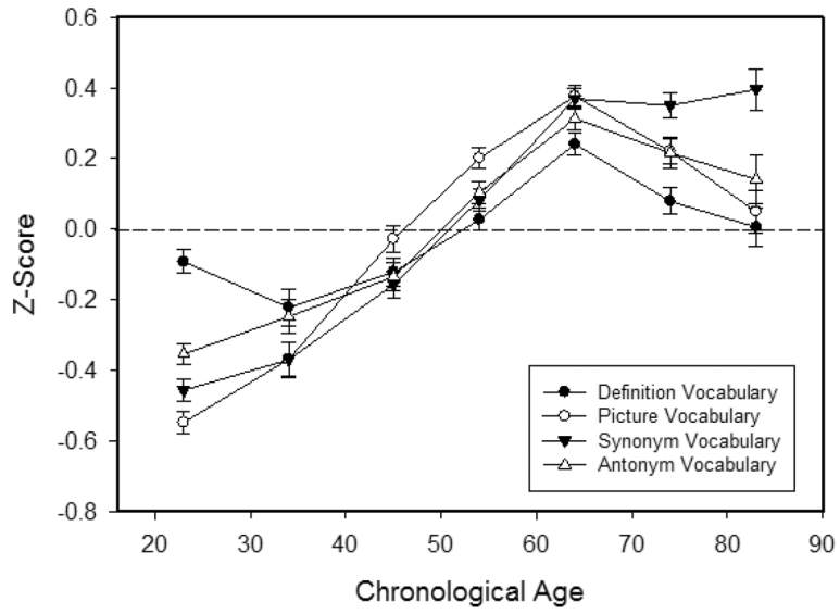
Figure 2. Means (and standard errors) of scores on four vocabulary tests on the first session of the first occasion by age decade. Definition vocabulary was assessed with the WAIS Vocabulary test.
