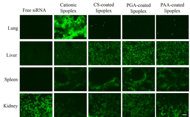
Fig. 5. Biodistribution of Cy5.5-siRNA at 1 h after intravenous administration by anionic polymer-coated lipoplexes into mice. Green signals indicate localization of Cy5.5-siRNA. Scale bar = 100 μm.
