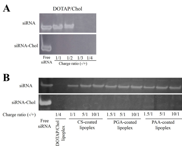
Fig. 2. Association of siRNA with cationic liposome after coating with various anionic polymers. (A) Cationic lipoplexes of 1 \mu g of siRNA or siRNA-Chol at various charge ratios (+/-) were analyzed by 18% acrylamide gel electrophoresis. Charge ratio (-/+) indicates the molar ratios of siRNA phosphate to DOTAP nitrogen. (B) Anionic polymer-coated lipoplexes of 1 \mu g of siRNA or siRNA-Chol at various charge ratios (-/+) were analyzed by 18% acrylamide gel electrophoresis. Charge ratio (-/+) indicates the molar ratios of sulfate and/or carboxylic acid of anionic polymers/DOTAP nitrogen.
