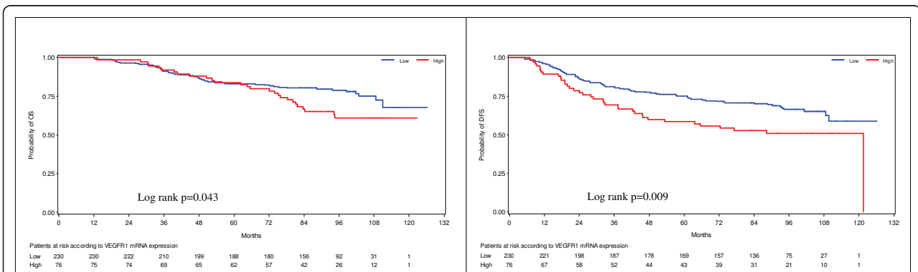
Figure 3 Kaplan-Meier curves according to VEGFR1 mRNA expression. High mRNA expression of VEGFR1 (above the 75 th percentile) was associated with significantly reduced OS (left) and DFS (right). DFS, disease-free survival; OS, overall survival; VEGFR1, vascular endothelial growth factor receptor 1.
