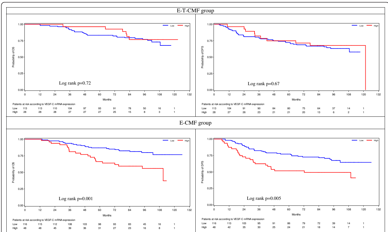
Figure 2 Kaplan-Meier curves according to VEGF-C mRNA expression and treatment. OS and DFS for patients with low VEGF-C mRNA expression (blue line) and high VEGF-C mRNA expression (red line) randomized in the E-T-CMF and E-CMF treatment groups. Interaction between VEGF-C mRNA expression and treatment group was significant for OS ( P = 0.019 ) and DFS ( P = 0.041 ). CMF, cyclophosphamide, methotrexate, fluorouracil; DFS, disease-free survival; OS, overall survival; VEGF-C, vascular endothelial growth factor C.
