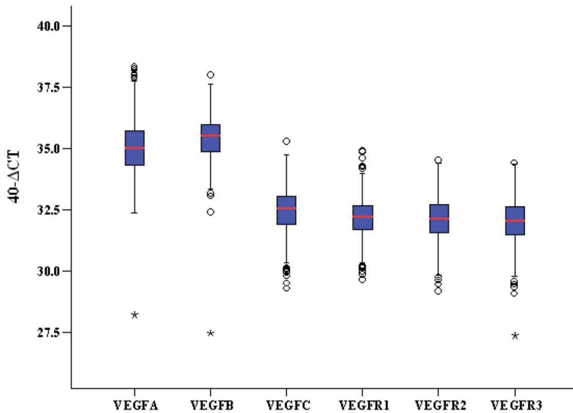
Figure 1 Distribution of mRNA expression values. Normalized mRNA expression values (40-delta CT) of all qRT-PCR evaluated VEGF family members are presented. CT, cycle threshold; VEGF, vascular endothelial growth factor.
