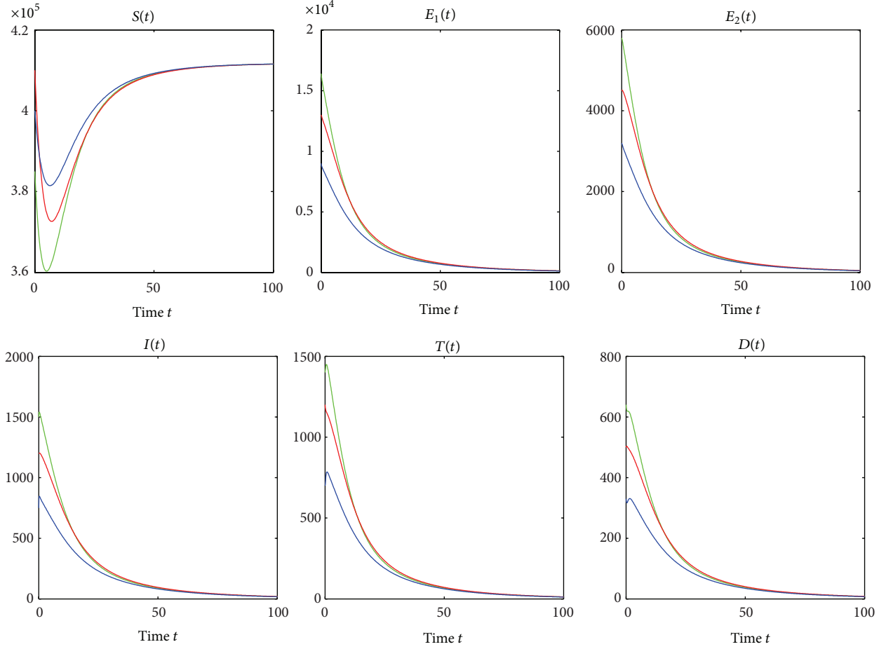
FIGURE 2: The global asymptotic stability of the disease-free equilibrium P_0 when R_{ii} = 0.9338 . The green line, the red line, and the blue line correspond to the initial values (3.85 \times 10^5, 1.64 \times 10^4, 5.8 \times 10^3, 1.5 \times 10^3, 1.4 \times 10^3, 640) , (4.1 \times 10^5, 1.3 \times 10^4, 4.5 \times 10^3, 1.2 \times 10^3, 1.2 \times 10^3, 500) , and (4 \times 10^5, 9 \times 10^3, 3.2 \times 10^3, 750, 700, 330) , respectively. \beta_2 is fixed as 0.00000035. Other parameter values can be seen in Table 1.
