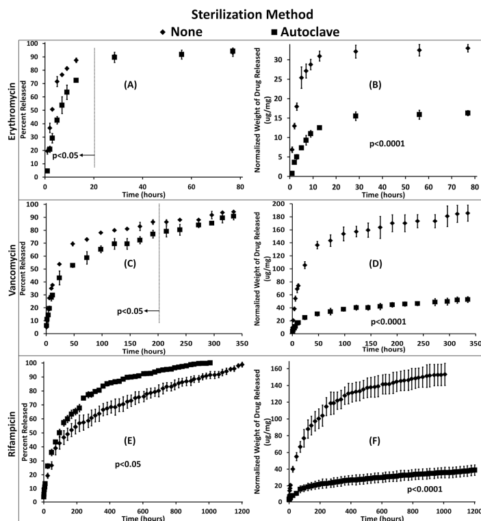
Fig. 4. Drug released from cyclodextrin:HDI polymers sterilized by autoclave compared to non-sterilized that were loaded with (A, B) erythromycin, (C, D) vancomycin, and (E, F) rifampicin after sterilization. (Left) The percentage of drug released slowed significantly after autoclaving ( p < 0.05 ), and (Right) the total amount of drug released was significantly lower in autoclaved polymers compared to non-sterilized controls ( p < 0.0001 ). Each drug releases at a different rate and therefore is presented on a different time scale.
