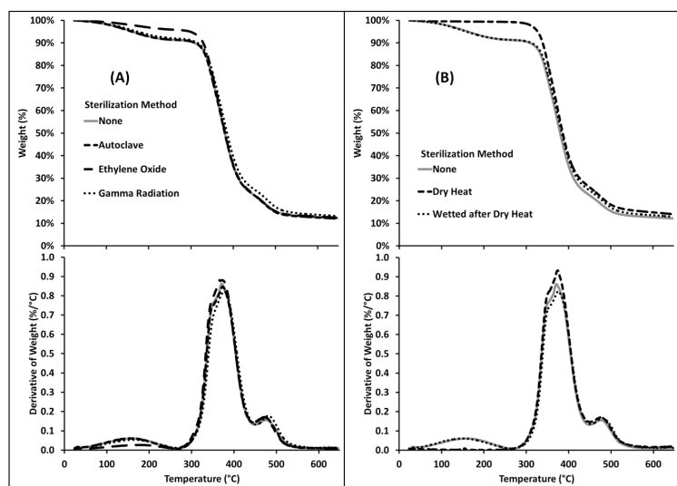
Fig 1. TGA data of cyclodextrin:HDI polymers showing that sterilization has minimal effect on the degradation profiles. Top: weight % vs. temperature. Bottom: Derivative of weight % vs. temperature. (a) Polymers sterilized by autoclave, ethylene oxide, and gamma radiation compared to a non-sterilized polymer. All four plots are identical, except less degradation is observed at 150°C in polymers sterilized by ethylene oxide due to reduced embedded water content. (b) After dry heat sterilization, no degradation exists at 150°C (because embedded water content is evaporated during the dry heat sterilization procedure), but the degradation peak returns after the polymer is wetted and dried overnight.
