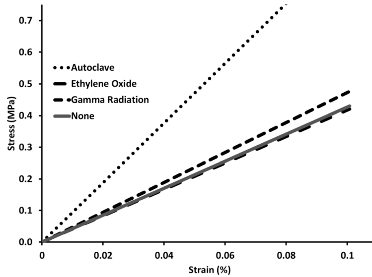
Fig. 3. Stress vs. strain plot from tensile tests comparing cyclodextrin:HDI polymers sterilized by gamma radiation, ethylene oxide, and autoclave with non-sterilized polymers to show a change in Young's modulus (tensile strength). A significant increase in tensile strength is observed in polymers sterilized by autoclave (N=5, p < 0.00001 , Table 2).
