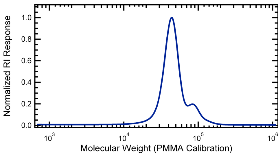
Figure 1. Normalized gel permeation chromatography trace of deprotected poly(N-isopropylacrylamide) product with a poly(methyl methacrylate)-equivalent molecular weight of 51.3 kg/mol and a polydispersity of 1.24.
