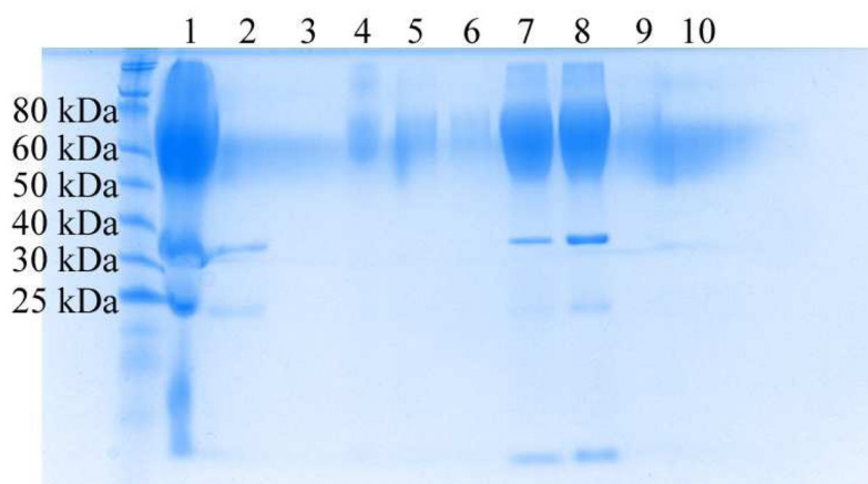
Figure 2. Denaturing SDS-PAGE gel showing purification of mCherryS131C-PNIPAM conjugate. The crude reaction mixture (lane 1) was purified by repeated precipitation of the conjugate using ammonium sulfate to remove unconjugated mCherryS131C. The discarded supernatants (lanes 2 and 3) contained most of the unconjugated mCherry. Next, metal affinity chromatography was used to remove excess PNIPAM. Minimal conjugate is lost from the column flow through (lane 4) and the two wash steps (lanes 5 and 6). The conjugate is then eluted in four fractions (lanes 7–10).
