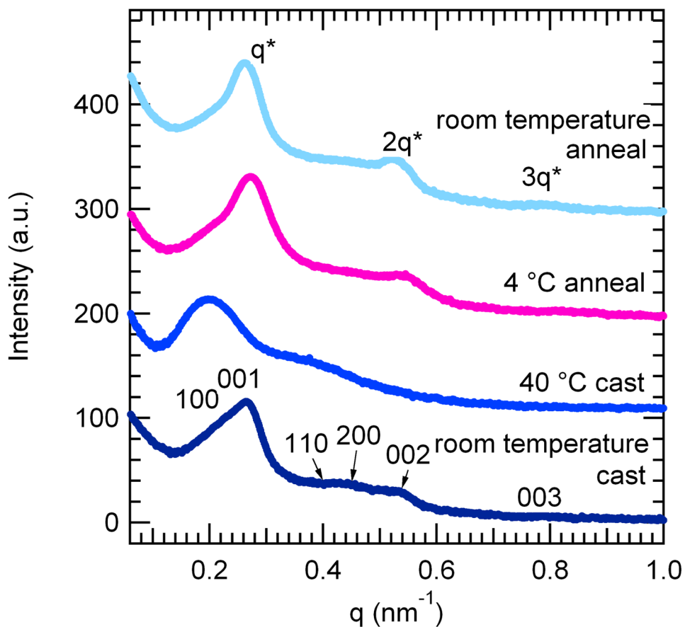
Figure 3. Small-angle x-ray scattering (SAXS) data of as-cast and solvent annealed mCherry-PNIPAM block copolymers. Samples were cast from both protein-selective (40 °C water) and nonselective (room temperature water) solvents. The materials form long-range ordered nanostructures with weak order. After solvent annealing in water, the samples transition to lamellar nanostructures with improved long-range order. Traces have been offset for clarity.
