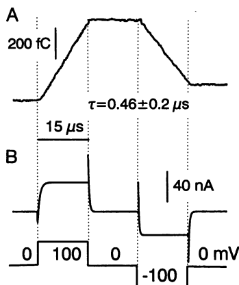
FIG. 1. A 1-MHz voltage clamp of calcium-activated chloride current in a giant Xenopus oocyte patch. Pipette resistance, 50 \Omega ; membrane capacitance, 5 pF; 100 mM CsCl on both sides. (A) Subtracted charge records or results with minus without 2 \mu\text{M} cytoplasmic free calcium. Voltage pulses were 15 \mu\text{s} . A fitted linear function plus an exponential corner function is plotted as a dotted line at each voltage with the data. The average time constant for adjustment of current to a new potential, \tau , was 0.46 \pm 0.2 \mu\text{s} (SEM, n = 4 ). (B) Membrane current, approximated as the first derivative of the functions fitted to the charge records.
