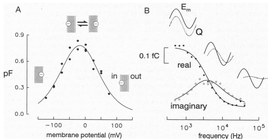
FIG. 2. Voltage and frequency dependence of the capacitance and admittance induced by a hydrophobic ion, dipicrylamine (DPA) (0.2 \mu\text{M} ) in a cardiac myocyte patch. (A) Voltage dependence of DPA-induced capacitance. Results are the subtraction of capacitance–voltage relations obtained in control solutions from relations obtained with 0.2 \mu\text{M} DPA on the cytoplasmic side. (B) Frequency scan of the DPA-induced charge signal in 1-MHz voltage clamp. Capacitance is monitored as the “real” component of the charge signal ( Q ) in phase with applied voltage ( E_m ). The “imaginary” component, measured 90^\circ from applied voltage, shows bell-shaped dependence on frequency. See text for description of data fits.
