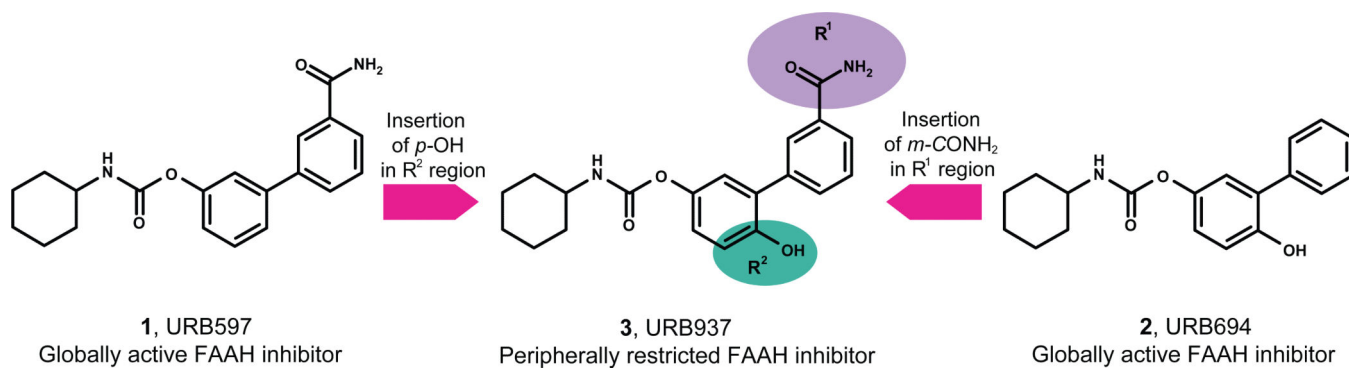
Figure 1. Design of peripherally restricted FAAH inhibitors.
