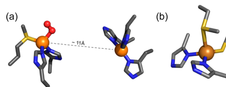
Figure 1. Copper enzymes/proteins with S-ligands: (a) Peptidylglycine- \alpha -hydroxylating monooxygenase (PHM), C–H oxygenation, (b) Azurin, electron transfer.
