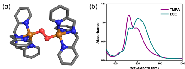
Figure 4. (a) Structure of [\{(\text{TMPA})\text{Cu}^{\text{II}}\}_2(\mu\text{-}1,2\text{-O}_2^{2-})\}^{2+}]^{2+} obtained from X-ray crystallography and (b) low-temperature UV–vis absorption spectra of [\{(\text{TMPA})\text{Cu}^{\text{II}}\}_2(\mu\text{-}1,2\text{-O}_2^{2-})\}^{2+}]^{2+} (purple) and [\{(\text{ESE})\text{Cu}^{\text{II}}\}_2(\mu\text{-}1,2\text{-O}_2^{2-})\}^{2+}]^{2+} (blue). 96,25
