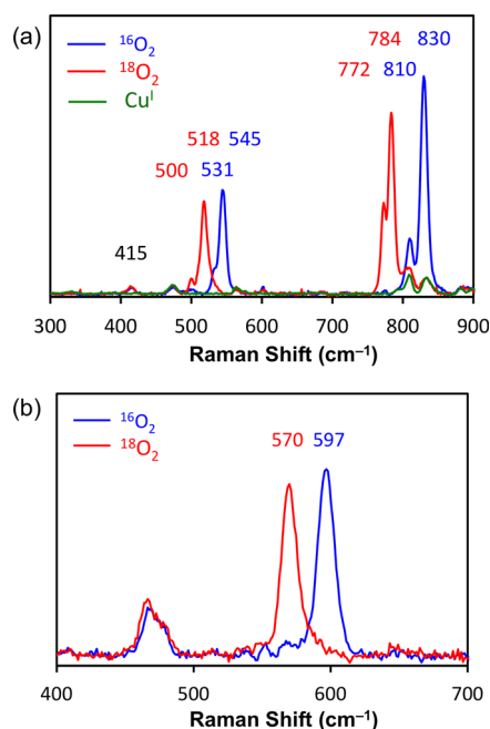
Figure 7. Resonance Raman spectra of 2 P (a) with 647 \text{ nm} excitation and 2 O (b) with 380 \text{ nm} excitation in MeTHF collected at 77 \text{ K} ; see text.
