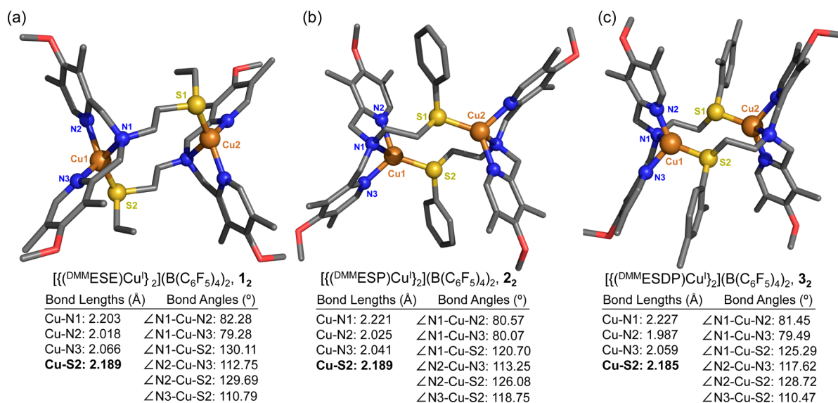
Figure 2. Representations of the dimeric Cu(I) complexes described in the crystal structures of (a) [ (DMM)ESE Cu] 2 (B(C 6 F 5 ) 4 ) 2 ( 1 2 ), (b) [ (DMM)ESP Cu] 2 (B(C 6 F 5 ) 4 ) 2 ( 2 2 ), and (c) [ (DMM)ESDP Cu] 2 (B(C 6 F 5 ) 4 ) 2 ( 3 2 ). Selected bond distances (Å) and bond angles (deg) are also listed. The H atoms and counterions were omitted for clarity.
