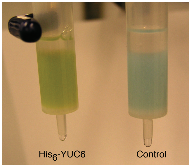
Figure 5. Purification of recombinant YUC6 with the flavin-cofactor bound. YUC6 tagged with His 6 at the N-terminus was expressed in E. coli and purified with Nickel NTA agrose. Note that the flavin cofactor in YUC6 gave the bright yellow color.
