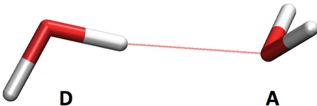
Figure 3. Water dimer as optimized with B3LYP/TZVP. The hydrogen bond donor (D) is on the left, the hydrogen bond acceptor (A) is on the right.
