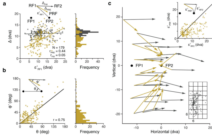
Figure 2. Shifting of FEF neuronal RFs prior to saccade onset a , The presaccadic shift amplitude ( \Delta_{PRE} ) as a function of the distance of RF1 from the saccade target (FP2) ( \epsilon'_{RF1} ) for 179 FEF RFs. The distance between RF1 and RF2 ( \Delta_{FIX} ) as a function of \epsilon'_{RF1} is shown for comparison. Lines denote linear regression fits. b , The angular deviation of the presaccadic RF shift from the remapping prediction ( \phi' ) as a function of \theta . c , Comparison of the population of presaccadic RF shifts (gold vectors) with the remapping prediction (gray vectors). Vectors were averaged within the 6 by 6 dva spatial bins depicted in the lower right along with the distribution of individual RF1s. Upper right plot shows the distances between the PRF and the saccade target compared with the distances between RF2 and the saccade target. Black line denotes the line of unity. Vector origins and endpoints are based on, respectively, RF1 and RF2 and RF1 and PRF.
