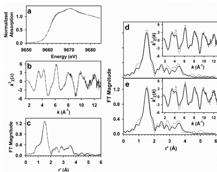
Figure 6. (left) Comparisons of the XAS data obtained for as-isolated (solid black line) and reconstituted (dashed grey line) ZnCA. The XANES spectra (a), k^3\chi(k) EXAFS spectra (b), and the Fourier transforms (c, k = 1.5 - 13.0 \text{ \AA}^{-1} ) are essentially superimposable. Fourier transforms of the unfiltered k^3\chi(k) EXAFS data (insets) of as-isolated CA (d) and reconstituted CA (e). Experimental data are represented by dotted lines, while best fits (given in bold in Table 2) are shown as solid black lines.
