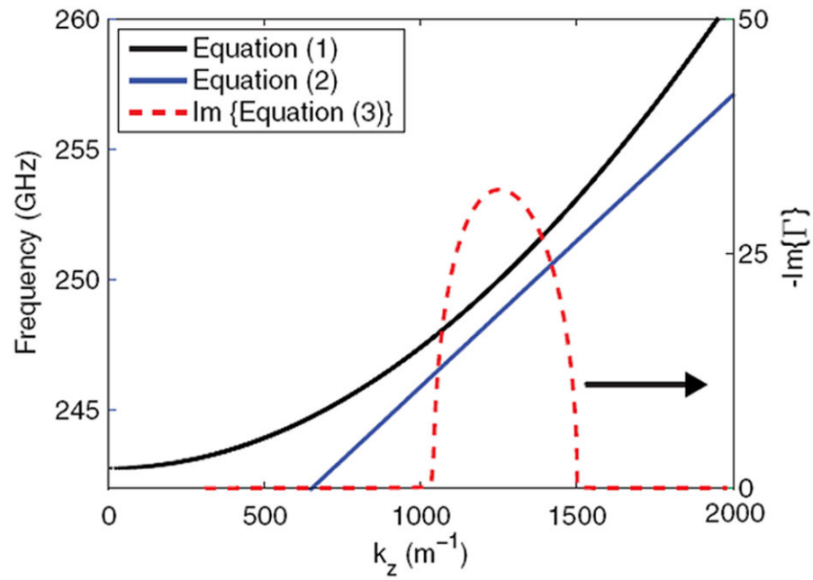
FIG. 1. (color online). Uncoupled and coupled dispersion relations for the waveguide mode and the electron beam for nominal operating conditions. Amplification would be observed when the imaginary part of \Gamma is nonzero.
