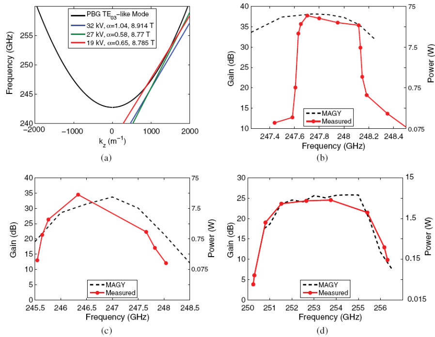
FIG. 5. (color online). (a) Dispersion relations [(1) and (2)] for three operating points with (b) 32 kV, 8.914 T, 0.345 A, 2.5% velocity spread and P_{in} = 7.5 mW; (c) 27 kV, 8.77 T, 0.225 A, 4% velocity spread and P_{in} = 7.5 mW; (d) 19.3 kV, 8.785 T, 0.4 A, 2% velocity spread and P_{in} = 15 mW.
