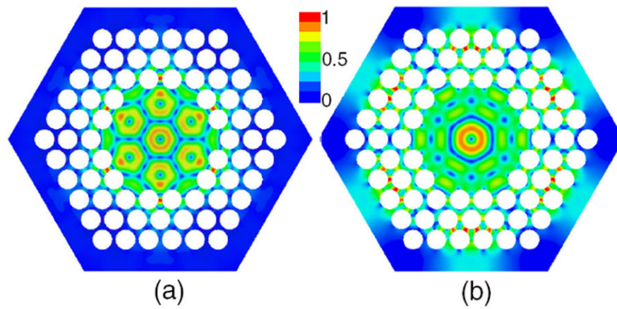
FIG. 2. (color online). Comparison between electric field of PBG waveguide modes with a cutoff frequency of (a) 242.7 GHz and (b) 212.1 GHz. The (a) operational TE 03 -like mode is well confined ( Q_{\text{diff}} = 1370 ) and (b) the lower-order mode is not confined ( Q_{\text{diff}} = 35 ). The white circles are stainless steel rods with lattice constants of a = 0.397 mm and a/b = 0.43 .
