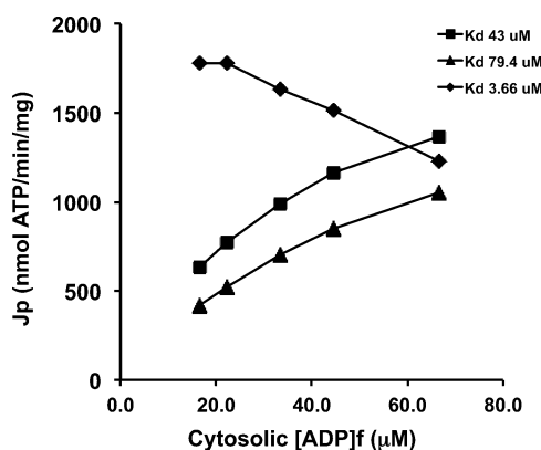
Figure 7. Data reported in Table 5 are graphically illustrated here. The rate of export of mitochondrial ATP by ANT ( J_{ANT} ) is simulated with the kinetic model of Metelkin et al. 10 at K_d\text{ADP} values of 3.66, 43.0, and 79.4 \mu\text{M} . These K_d\text{ADP} values correspond to deacetylated ANT1, the observed data of Glancy et al. 25 in isolated mitochondria, and ANT1 acetylated at Lys23, respectively. See the text for further discussion.
