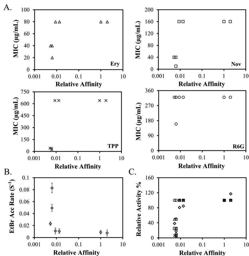
Figure 4. Correlation between AcrB trimer affinity and substrate efflux activity. (A) MIC of four different AcrB substrates determined for BW25113 \Delta acrB containing a plasmid encoded wild-type AcrB or AcrB mutants plotted against their relative affinity. Substrates tested were Ery (triangles), TPP (crosses), R6G (circles), and Nov (squares). (B) EtBr accumulation rate of BW25113 \Delta acrB containing a plasmid encoded wild-type AcrB or AcrB mutants plotted against their relative affinity. Each measurement was repeated at least three times. The average value and standard deviations are shown. (C) Normalized MIC values and EtBr accumulation rate (diamonds) plotted against the relative trimer affinity. The same symbols were used for Ery, TPP, R6G, and Nov as those used in panel A.
