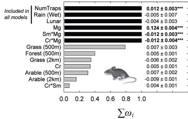
Figure 4. The model averaged terms (from selected models with \Delta AICc \leq 2 ) for models of the abundance of (a) Crocidura russula (Cr) (b) Sorex minutus (Sm) (c) Myodes glareolus (Mg) and (d) Apodemus sylvaticus (As). Bars show the relative importance of each term (ranked in order of the sum of their Akaike weights, \Sigma\omega_i ). Black bars indicate terms in the best-approximating model ( \Delta AICc = 0 ). NumTraps, Rain and Lunar were included in all models to control for confounding influences. Standardized regression coefficients ( \beta ) \pm 1 standard error (SE) are shown to the right of each bar. Significance levels from the best-approximating model are indicated as * p < 0.1 , * p < 0.05 , ** p < 0.01 and *** p < 0.001 , and significant terms at p < 0.05 are shown in bold. The R^2 values of observed versus fitted values for each best approximating model are 0.53, 0.22, 0.28 and 0.90 for C. russula , S. minutus , M. glareolus and A. sylvaticus , respectively. doi:10.1371/journal.pone.0100403.g004
