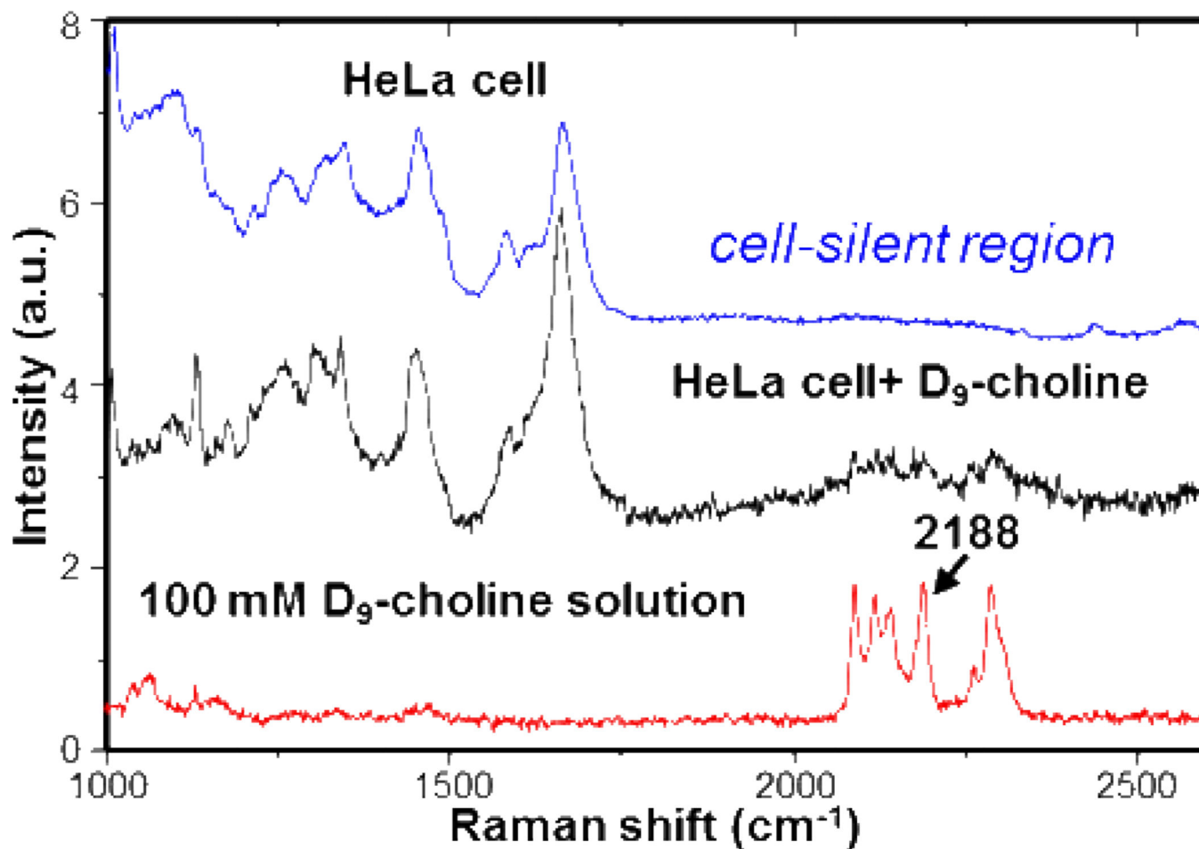
Figure 2. Spontaneous Raman spectra of HeLa cells supplemented with (black) and without (blue) D 9 -choline and 100 mM D 9 -choline (red) in phosphate buffered saline (PBS) solution. The 2188 cm -1 peak within the cell-silent Raman region is chosen for SRS imaging.
