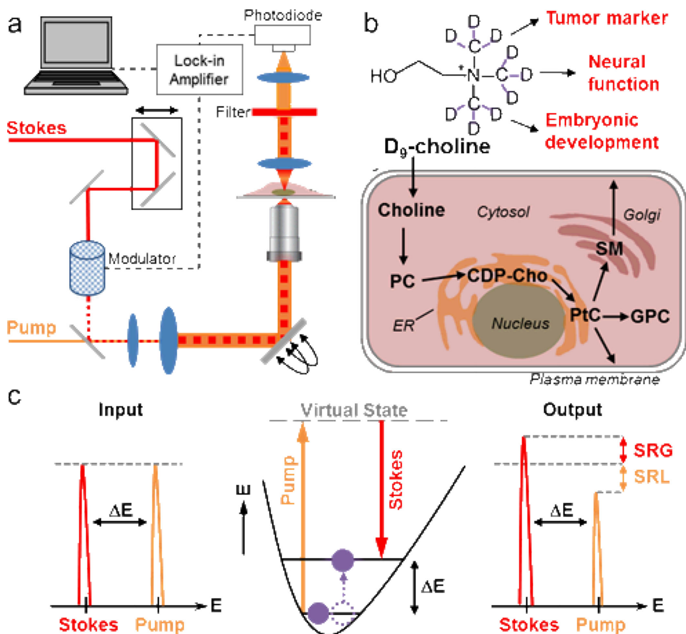
Figure 1. Stimulated Raman scattering (SRS) imaging of choline metabolites through metabolic incorporation of deuterated D 9 -choline. (a) Set up of SRS microscope. Spatially and temporally overlapped Stokes and pump beams lead to selective vibrational activation within the sample under the resonant condition. (b) Incorporation of D 9 -choline in the cellular pool of choline metabolites serves as a metabolic biomarker in tumor progression, brain function and embryonic development. (c) Energy diagram together with the input and output laser spectra of SRS.
