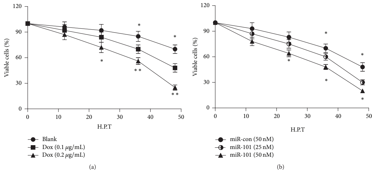
FIGURE 5: MiR-101 deteriorates the Dox-induced cell viability reduction. (a) Viability of U-2 cells after Dox treatment with 0, 0.1, or 0.2 \mu\text{g}/\text{mL} . (b) Viability of U-2 cells after 0.1 \mu\text{g}/\text{mL} Dox treatment and the transfection with 25 or 50 nM miR-101 mimics or 50 nM miR control ( * P < 0.05 ; ** P < 0.01 ). All results were from three independently performed experiments.
