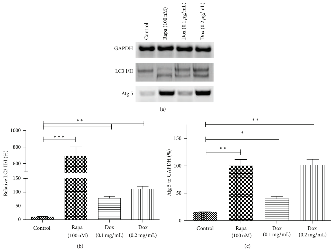
FIGURE 2: Dox promotes the conversion of LC3-I to LC3-II and increases Atg 5 expression. (a) Western blotting results of U-2 OS cells with Dox (0.1 or 0.2 \mu\text{g}/\text{mL} ) or Rapa (100 nM) treatment. (b) Quantitative analysis of the conversion of LC3-I to LC3-II in various groups. (c) Quantitative analysis of the relative Atg 5 expression to GAPDH in U-2 OS cells after various treatments. Statistical significance shown as * P < 0.05 , ** P < 0.01 , and *** P < 0.001 . All results were from three independently performed experiments.
