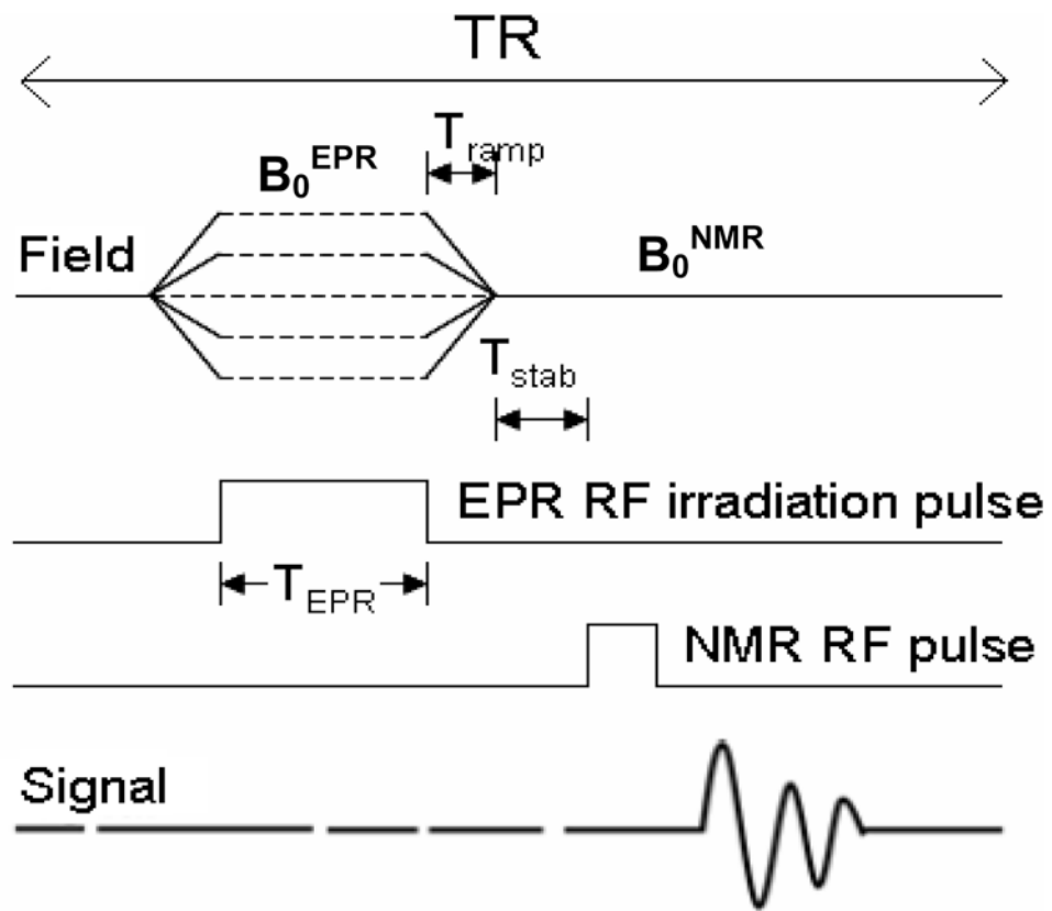
Fig.4. FC-DNP spectroscopy pulse sequence diagram
