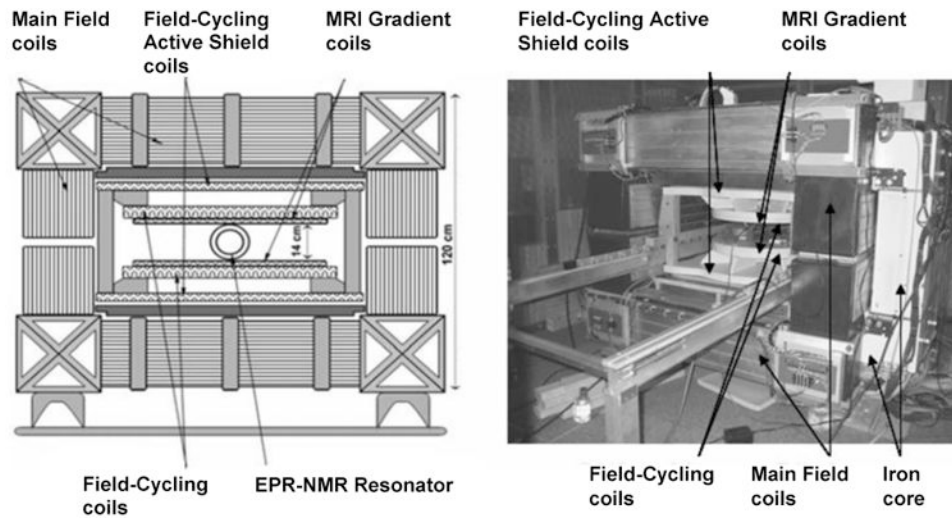
Fig.2. Mechanical layout and photograph of the variable-field DNP spectroscopy system
