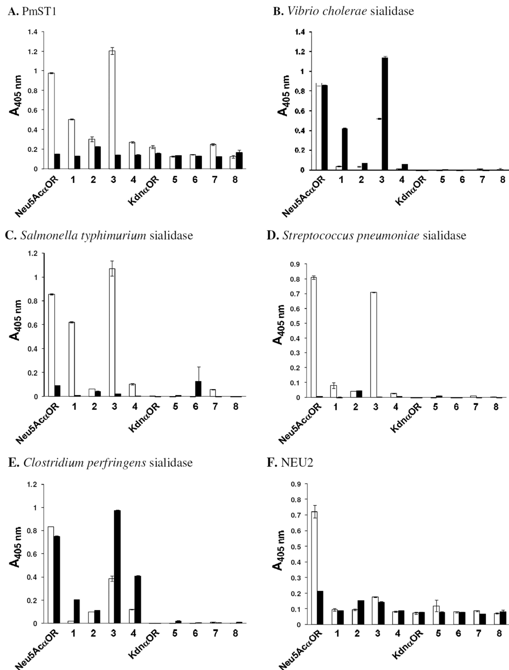
Figure 3. Sialidase substrate specificity studies using \alpha 2–3- ( 1b–8b ) and \alpha 2–6-linked ( 1c–8c ) sialyl Gal \beta pNP containing C7-modified sialic acids. Neu5Aca \alpha 2–3/Gal \beta 3pNP and Kdn \alpha 2–3/Gal \beta 3pNP are used as controls. Results using \alpha 2–3-linked sialosides as substrates are shown in white bars and results using \alpha 2–6-linked sialosides as substrates are shown in black bars.
