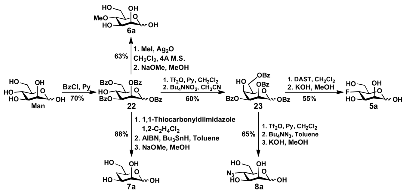
Scheme 4. Synthesis of C4-modified mannose derivatives 5a–8a .
