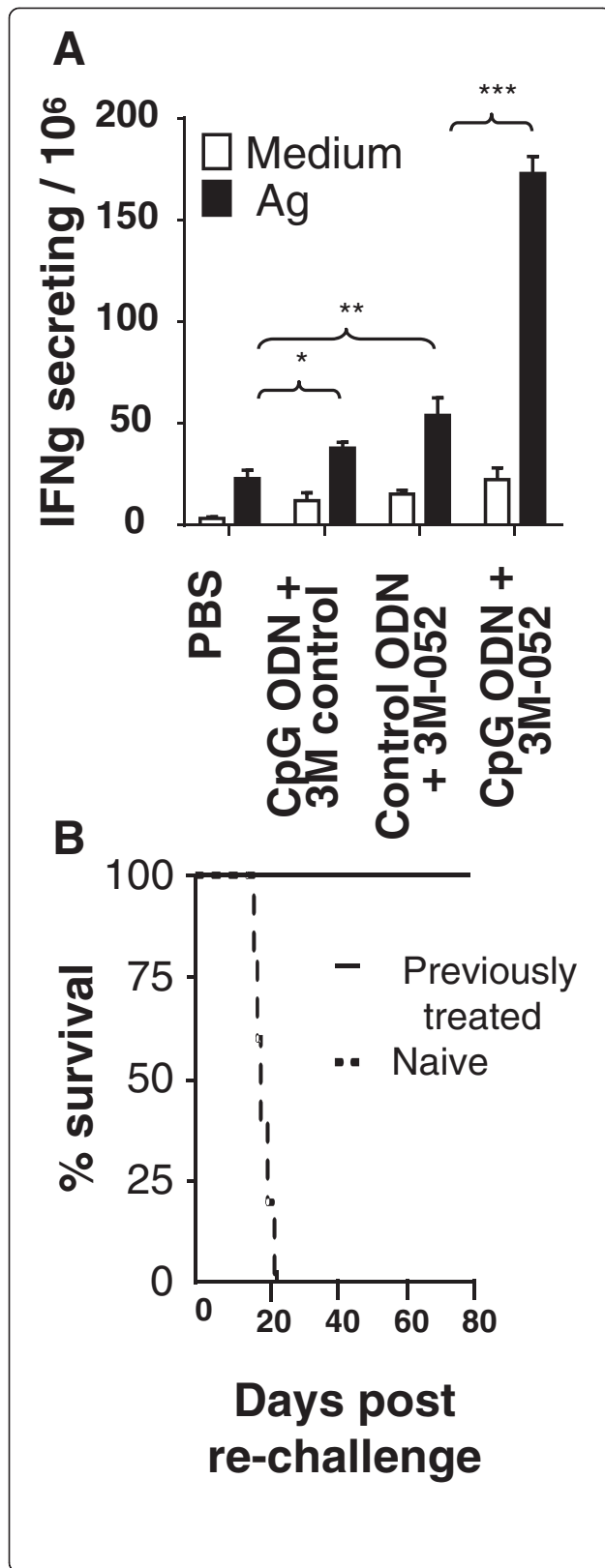
Figure 7 TLR agonist therapy induces persistent immunity. 10 5 CT26 cells were implanted into the flank of syngeneic BALB/c mice. Large established tumors (≈800 mm 3 in volume) were treated as described in Figure 5. A ) Cells from the tumor draining LN were isolated one day after the third treatment, stimulated ex vivo with AH-1 peptide, and monitored for IFN \gamma secretion by ELISpot assay. Results represent the mean + SD of 4 independently studied mice/group. B ) Mice cured of their CT26 tumors by treatment with CpG ODN plus 3M-052 (a cure being defined as being free of detectable tumor for \geq 2 months after the cessation of therapy) were re-challenged with 10 6 CT26 cells. Their survival compared to naive mice challenged with the same tumor dose is shown (N = 6 mice/group). *, p < 0.05; **, p < 0.01, ***, p < 0.001.
