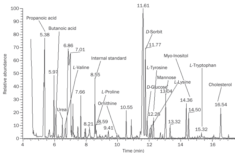
Figure 1. A GC/MS chromatograph of plasma samples obtained from a control rat. Some typical metabolites and the internal standard are labeled.
