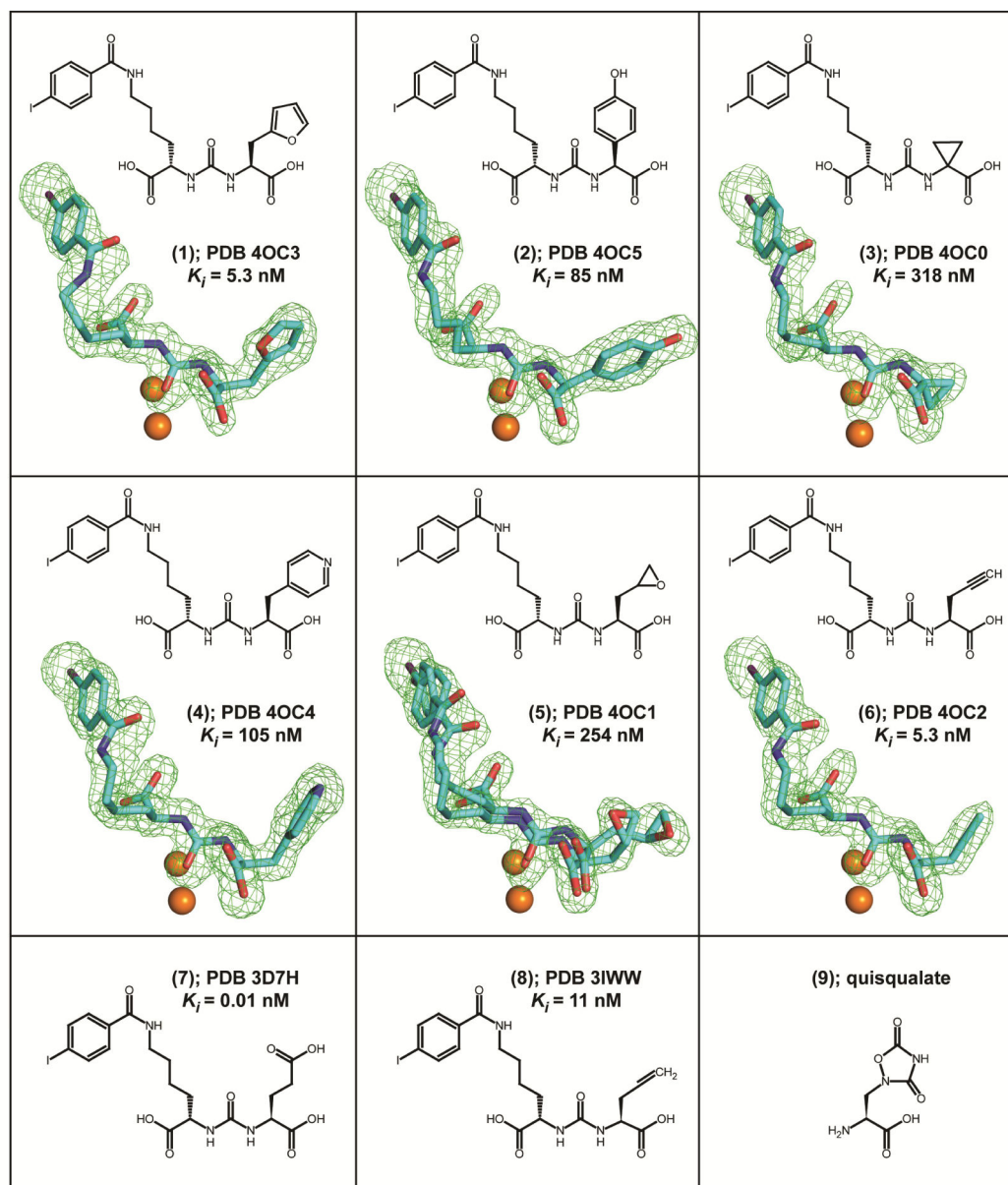
Figure 1. Chemical formulas, PDB codes, and inhibition constants of inhibitors used in this study. Fo-Fc maps (green) for individual inhibitors are contoured at 3.0 \sigma and modeled inhibitors are shown in stick representation with atoms colored cyan (carbon), red (oxygen), blue (nitrogen), and violet (iodine). The active-site zinc ions are shown as orange spheres.
