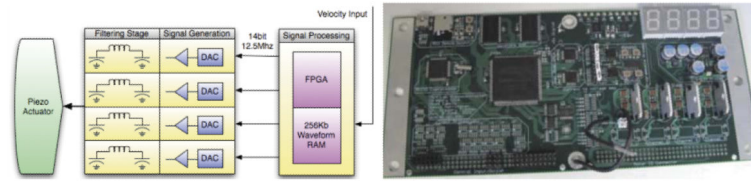
Figure 3. (Left) piezoelectric actuator driver architecture using FPGA generated waveform, (right) the piezoelectric driver board prototype, a key aspect of generating the low noise high precision motion.
