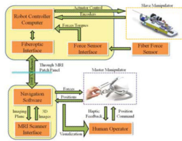
Figure 1. (Left) System architecture for the master - slave haptic interface. The fiber optic force sensor and robot are placed near the iso-center of the MRI scanner, the master manipulator is connected to the navigation software interface, and the two are couple through the robot controller in the scanner room using a fiber optic network connection. (right) The robot prototype in the bore of a 3T MRI scanner with a phantom.
