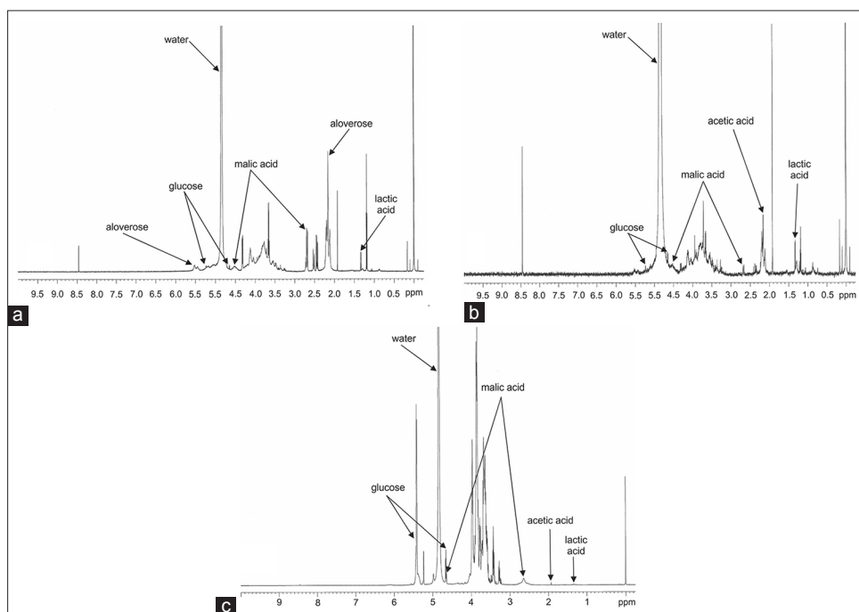
Figure 3: 1 H-NMR spectra of A. vera (a), A. marlothii (b) and A. ferox (c) precipitated gel materials
