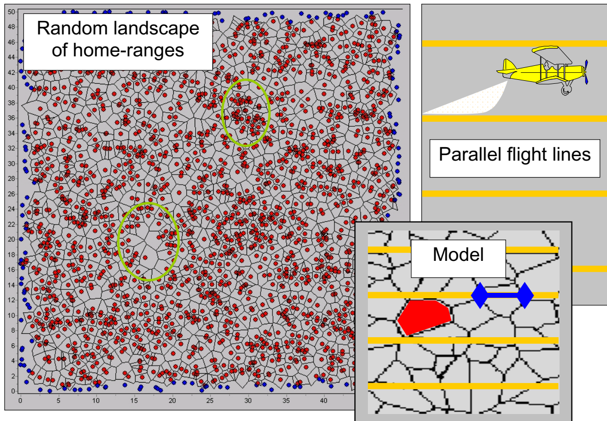
Figure 2 Schematic representation of the model Schematic representation of the components of the model: Randomly generated landscape of fox group home-ranges (including high and low density areas), the parallel flight lines randomly intersected with the 'fox landscape', and the measurements in the model (i) length of flight line segment in each polygon, (ii) number of empty polygons.
