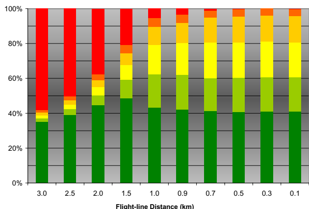
Figure 6 The effect of varying flight line distance The effect of varying flight line distance (i.e. management strategy) on the distribution of absolute bait numbers in the individual fox groups under the field strategy (pBaitDens = 20; mean fox group area ~1 km 2 ). Bar segments depict the percentage of spatial units with a particular number of baits (red 0; orange 1–5; light orange 6–10; yellow 11–15; green 16–20; dark green > 20 baits). Very small flight line distances cannot improve the ground pattern further, as small sized home-ranges can only contain a maximum number of baits even with perfectly uniform distribution.
