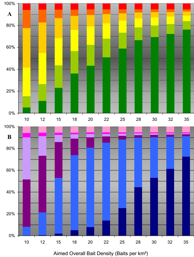
Figure 5 The effect of varying bait density The effect of varying bait density (i.e. management aim) on the distribution of absolute bait numbers in the individual fox group under the field strategy (pLineDist = 1 km; mean fox group area ~1 km 2 ). (a) Bar segments depict the percentage of spatial units with a particular number of baits (red 0; orange 1–5; light orange 6–10; yellow 11–15; green 16–20; dark green > 20 baits). (b) Bar segments depict frequencies of the relative deviation of the resulting local bait density from the aimed density of the campaign (pink -100% to -75%; lilac -74% to -50%; aubergine -49% to -25%; blue -25% to +50%; dark blue above +50% deviation of management aim of 20 b.p.km 2 ).
