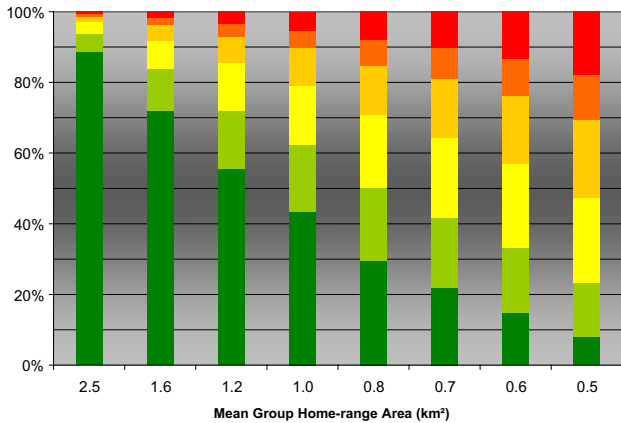
Figure 4 The effect of group home-range size The effect of mean area of family group home-range (i.e. fox density) on the distribution of absolute bait numbers in individual fox groups under the field strategy (pBaitDens = 20; pLineDist = 1 km). Bar segments depict the percentage of spatial units with a particular number of baits (red 0; orange 1–5; light orange 6–10; yellow 11–15; green 16–20; dark green > 20 baits).
