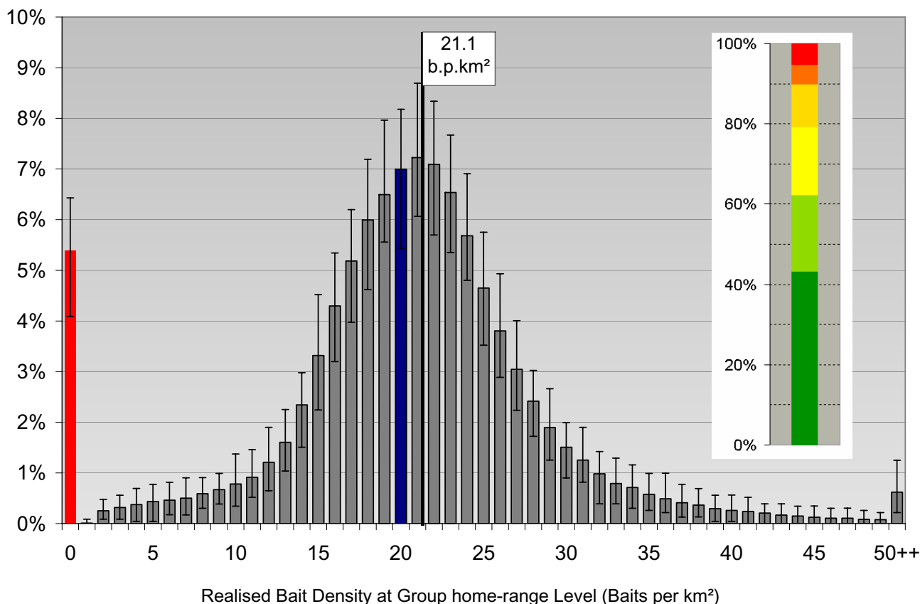
Figure 3 Frequency distribution of local bait densities Full frequency distribution of local bait densities found under the reference or field scenario (pBaitDens = 20; pLineDist = 1 km; pN = 2500; MaxX*MaxY = 2500 km 2 ), whiskers represent MIN and MAX of 100 repetitions. The segments of the inserted bar diagram illustrate the percentage of spatial units with a particular number of baits (red 0; orange 1–5; light orange 6–10; yellow 11–15; green 16–20; dark green > 20 baits). Management aim of 20 b.p.km 2 is exceeded on the group home-range level where mean bait density is measured as 21.1 b.p.km 2 .
