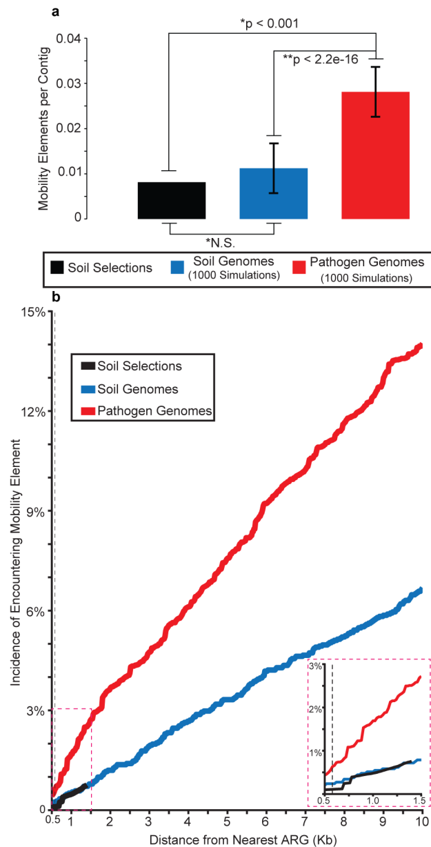
Figure 4. Pathogen ARGs show higher HGT potential than soil ARGs. (a) Mobility elements syntenic with ARGs are proportionally higher in pathogens than soil genomes or soil functional selections. (*) indicates significance determined from 1000 Monte Carlo simulations; (**) indicates significance determined by Student's T test. Error bars depict two standard deviations from mean. (b) Pathogens show significantly increased HGT potential relative to soil genomes and soil selections at all distances (20bp intervals) greater than 580bp (dashed line, p < 0.05 , Fisher's exact test). Inset depicts mobility elements encountered within 1.5Kb of ARGs, demonstrating that data from soil selections resembles soil genomes.
