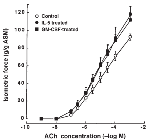
Figure 8 Comparison of airway constrictor responses to ACh in isolated paired ASM segments in the absence ( open circles ) and presence of 24-h exposure to maximum effective concentrations of IL-5 ( filled circles ) and GM-CSF ( filled squares ). Relative to controls, both the T_{max} and ED_{50} values to ACh were significantly enhanced in the presence of IL-5 and GM-CSF. Data represent mean \pm SE values from six paired experiments.
