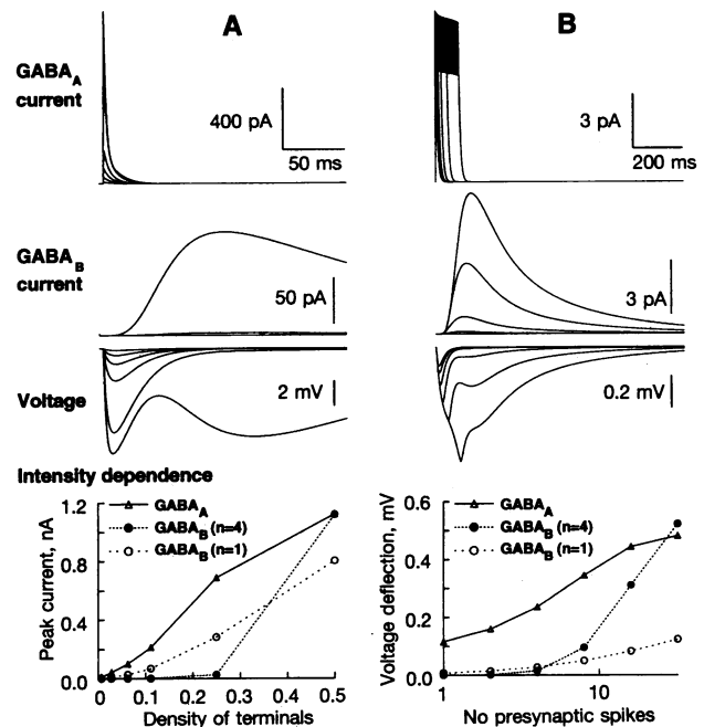
FIG. 3. Dependence of GABA A - and GABA B -mediated synaptic responses on the pattern of presynaptic stimulation. The GABA A current, the GABA B current, the postsynaptic potential, and the intensity dependence graph are arranged from top to bottom. (A) Dependence on the density of co-releasing terminals. Successive traces in each graph indicate the total postsynaptic current and voltage after a single presynaptic spike occurring simultaneously in 1, 4, 9, 16, 36, and 72 terminals (in a 144-compartment geometry). (B) Dependence on the number of presynaptic spikes occurring at a single synapse. In this case, the successive traces in each graph were obtained from trains of 1, 2, 4, 8, 16, and 32 presynaptic spikes at 300 Hz. (Bottom) Intensity dependence of GABA B responses are compared for single ( n = 1 ) and multiple ( n = 4 ) G-protein binding sites. GABA B current is scaled 10 times in A , and abscissa in B is in a logarithmic scale.
