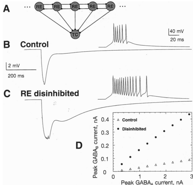
FIG. 4. Enhancement of the GABA B response in TC cells through disinhibition in the RE nucleus. (A) Connectivity: a simple network of RE cells was simulated with GABA A receptor-mediated synaptic interactions. All RE cells project to a single TC cell with synapses containing both GABA A and GABA B receptors. Models of the RE cells were taken from ref. 30. (B) In control conditions, the bursts generated in RE cells by stimulation have 2–8 spikes ( Inset ) and evoke in TC cells a GABA A -dominated IPSP with a small GABA B component. (C) When GABA A receptors are suppressed in RE, the bursts become much larger ( Inset ) and evoke in TC cells a stronger GABA B component. (D) Peak GABA A versus peak GABA B current for increasing numbers of RE cells stimulated.
